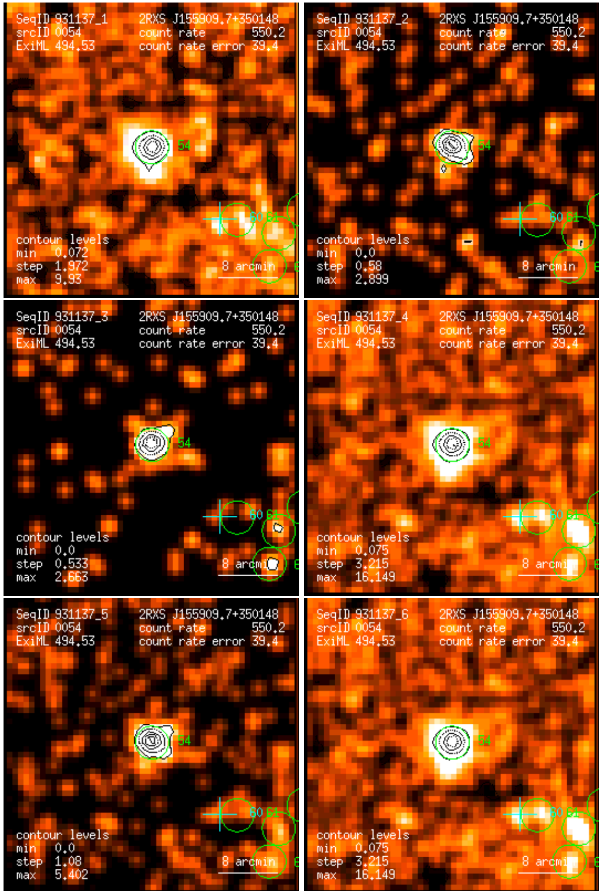
Figure 54: RASS 931137: detection 0054: band rate images, Gaussian filter: (1) PSPC channels 11 – 41, (2) 52 – 90, (3) 91 – 201, (4) 11 – 235, (5) 52 – 201, (6) 11 – 201. Broad band rates in counts/ks. Band rate contour levels in counts/ks/arcmin 2 .
