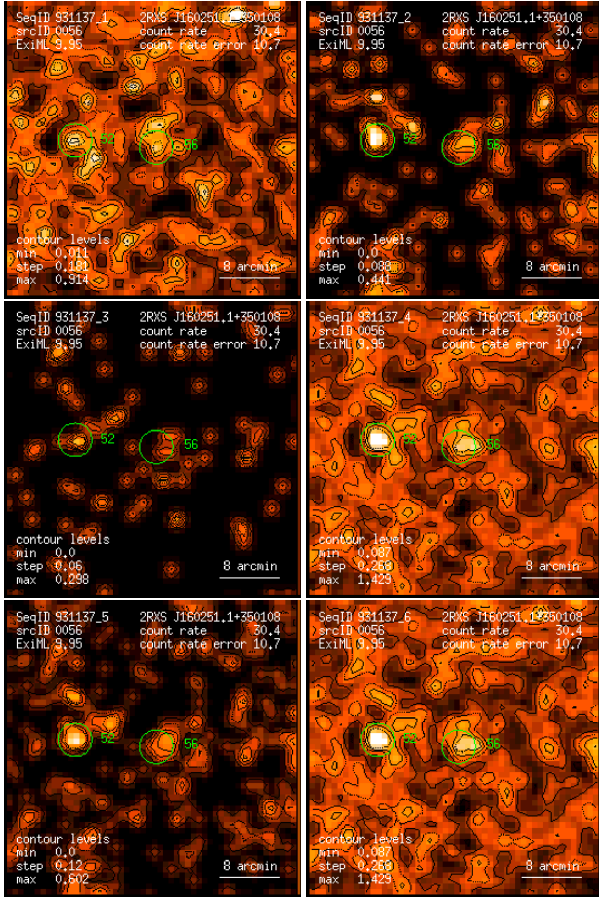
Figure 56: RASS 931137: detection 0056: band rate images, Gaussian filter: (1) PSPC channels 11 – 41, (2) 52 – 90, (3) 91 – 201, (4) 11 – 235, (5) 52 – 201, (6) 11 – 201. Broad band rates in counts/ks. Band rate contour levels in counts/ks/arcmin 2 .
