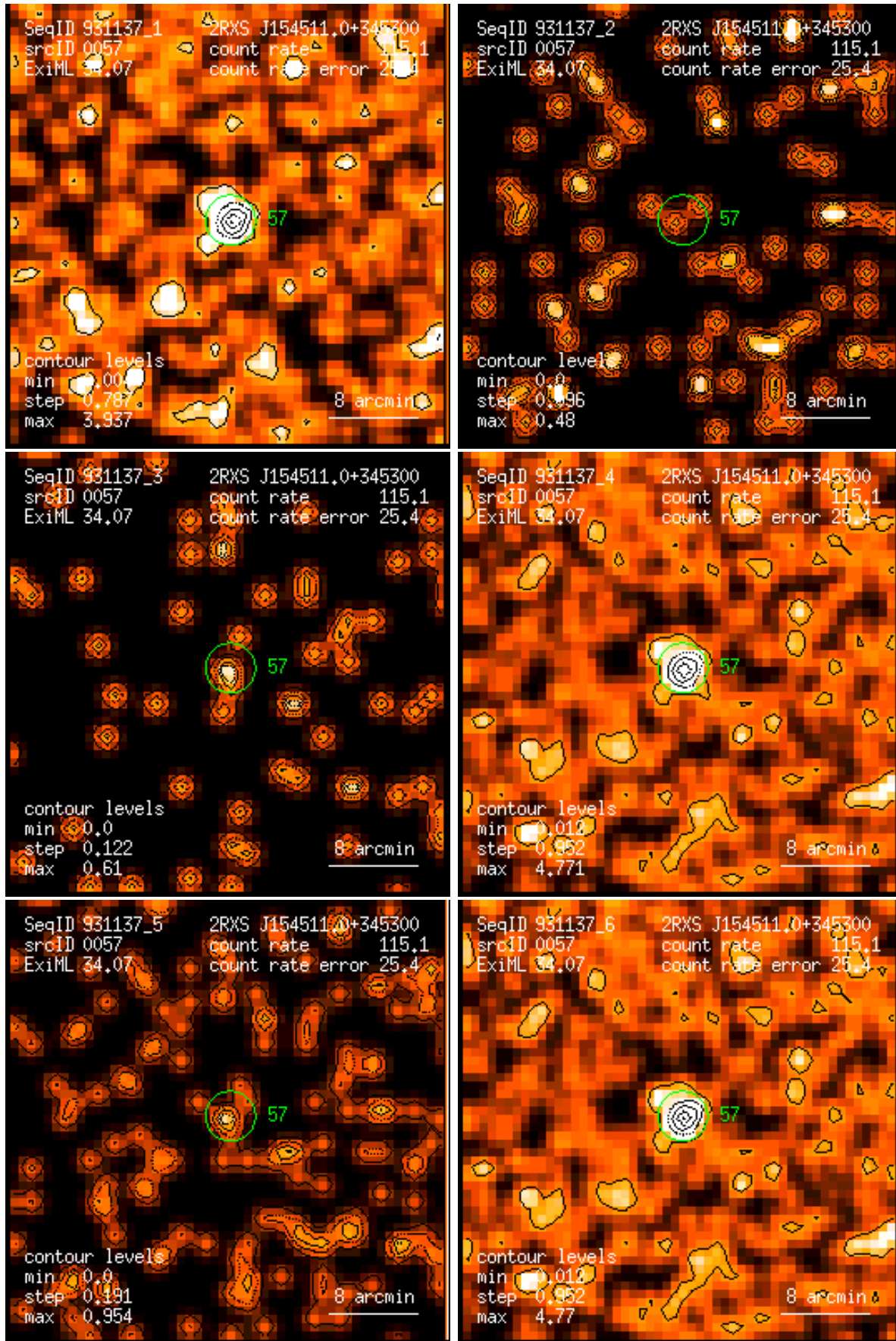
Figure 57: RASS 931137: detection 0057: band rate images, Gaussian filter: (1) PSPC channels 11 – 41, (2) 52 – 90, (3) 91 – 201, (4) 11 – 235, (5) 52 – 201, (6) 11 – 201. Broad band rates in counts/ks. Band rate contour levels in counts/ks/arcmin 2 .
