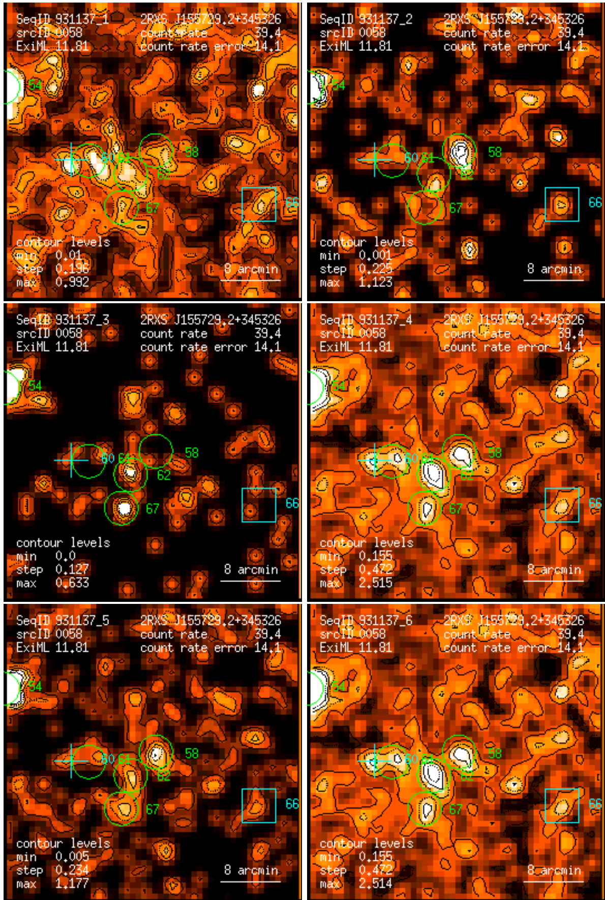
Figure 58: RASS 931137: detection 0058: band rate images, Gaussian filter: (1) PSPC channels 11 – 41, (2) 52 – 90, (3) 91 – 201, (4) 11 – 235, (5) 52 – 201, (6) 11 – 201. Broad band rates in counts/ks. Band rate contour levels in counts/ks/arcmin 2 .
