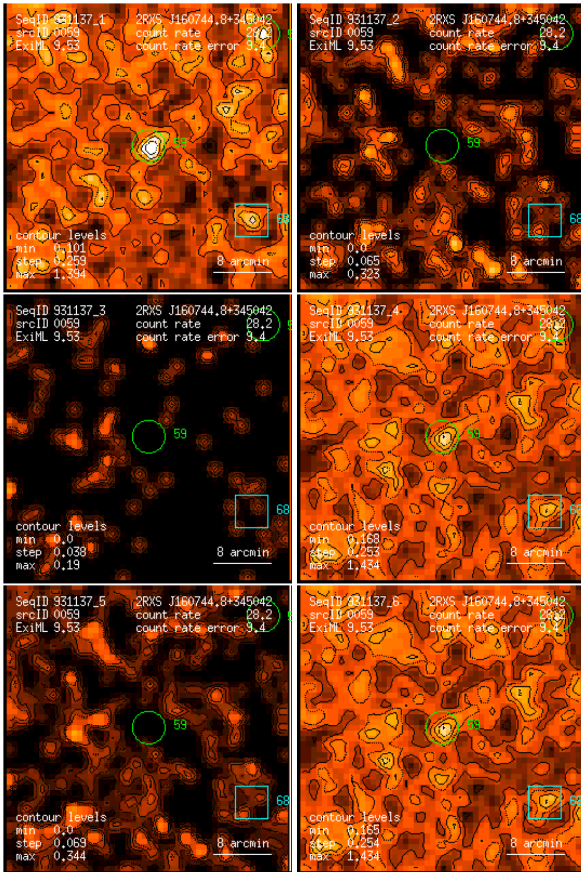
Figure 59: RASS 931137: detection 0059: band rate images, Gaussian filter: (1) PSPC channels 11 – 41, (2) 52 – 90, (3) 91 – 201, (4) 11 – 235, (5) 52 – 201, (6) 11 – 201. Broad band rates in counts/ks. Band rate contour levels in counts/ks/arcmin 2 .
