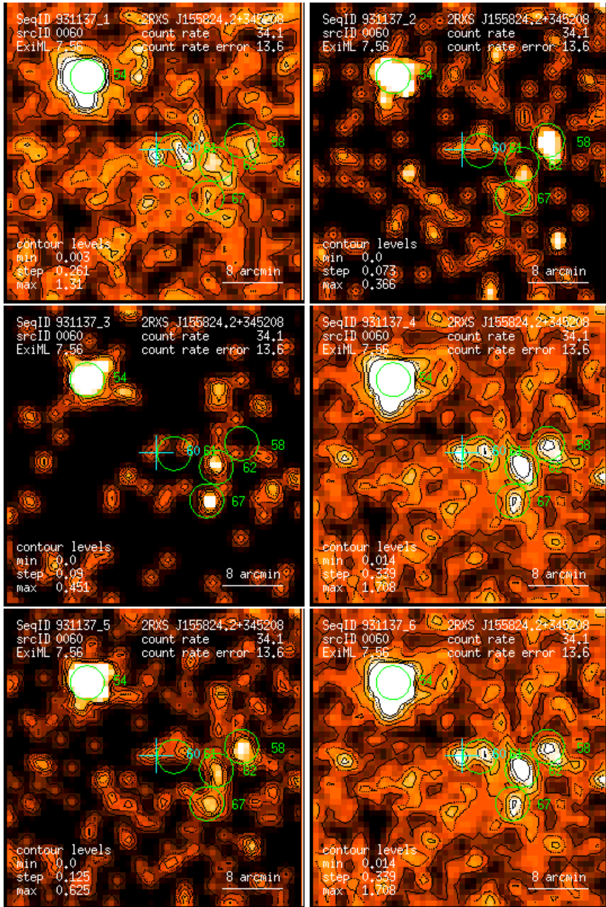
Figure 60: RASS 931137: detection 0060: band rate images, Gaussian filter: (1) PSPC channels 11 – 41, (2) 52 – 90, (3) 91 – 201, (4) 11 – 235, (5) 52 – 201, (6) 11 – 201. Broad band rates in counts/ks. Band rate contour levels in counts/ks/arcmin 2 .
