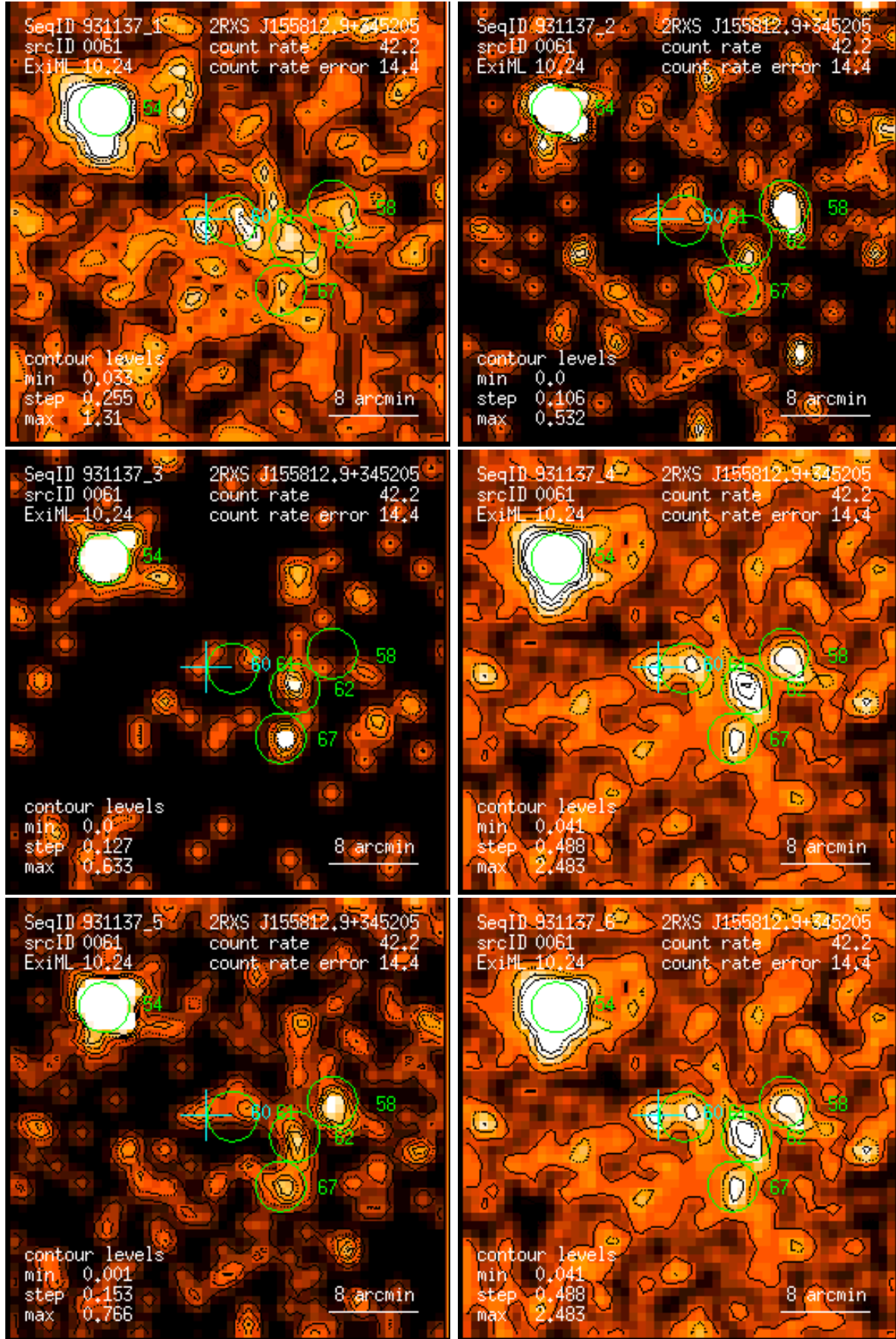
Figure 61: RASS 931137: detection 0061: band rate images, Gaussian filter: (1) PSPC channels 11 – 41, (2) 52 – 90, (3) 91 – 201, (4) 11 – 235, (5) 52 – 201, (6) 11 – 201. Broad band rates in counts/ks. Band rate contour levels in counts/ks/arcmin 2 .
