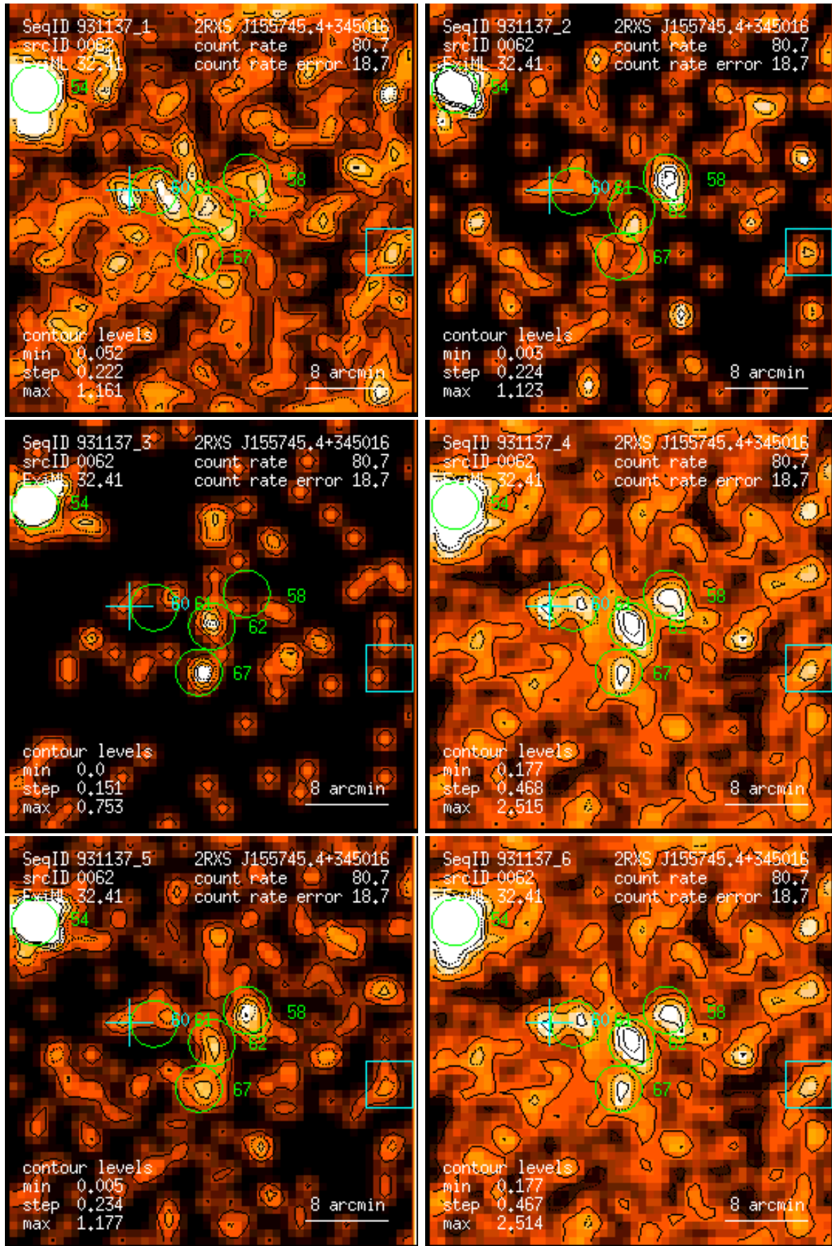
Figure 62: RASS 931137: detection 0062: band rate images, Gaussian filter: (1) PSPC channels 11 – 41, (2) 52 – 90, (3) 91 – 201, (4) 11 – 235, (5) 52 – 201, (6) 11 – 201. Broad band rates in counts/ks. Band rate contour levels in counts/ks/arcmin 2 .
