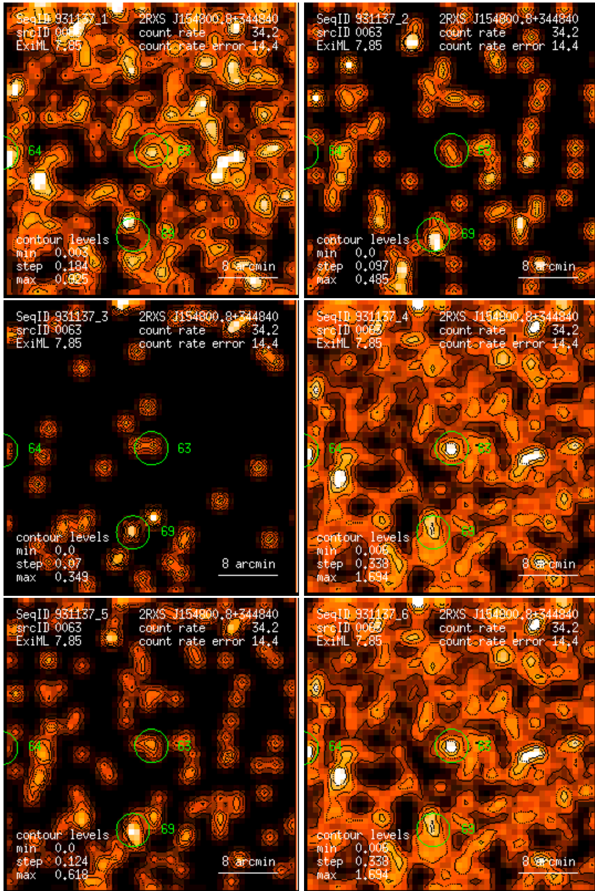
Figure 63: RASS 931137: detection 0063: band rate images, Gaussian filter: (1) PSPC channels 11 – 41, (2) 52 – 90, (3) 91 – 201, (4) 11 – 235, (5) 52 – 201, (6) 11 – 201. Broad band rates in counts/ks. Band rate contour levels in counts/ks/arcmin 2 .
