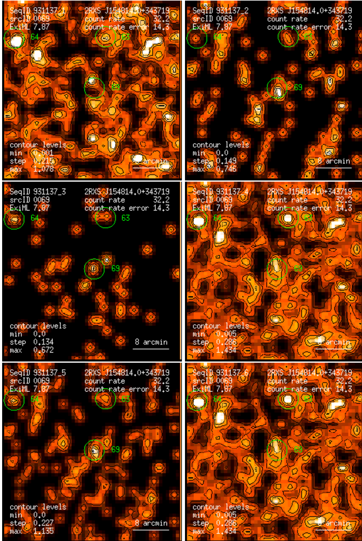
Figure 69: RASS 931137: detection 0069: band rate images, Gaussian filter: (1) PSPC channels 11 – 41, (2) 52 – 90, (3) 91 – 201, (4) 11 – 235, (5) 52 – 201, (6) 11 – 201. Broad band rates in counts/ks. Band rate contour levels in counts/ks/arcmin 2 .
