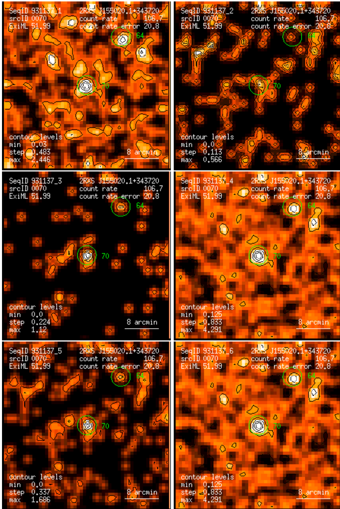
Figure 70: RASS 931137: detection 0070: band rate images, Gaussian filter: (1) PSPC channels 11 – 41, (2) 52 – 90, (3) 91 – 201, (4) 11 – 235, (5) 52 – 201, (6) 11 – 201. Broad band rates in counts/ks. Band rate contour levels in counts/ks/arcmin 2 .
