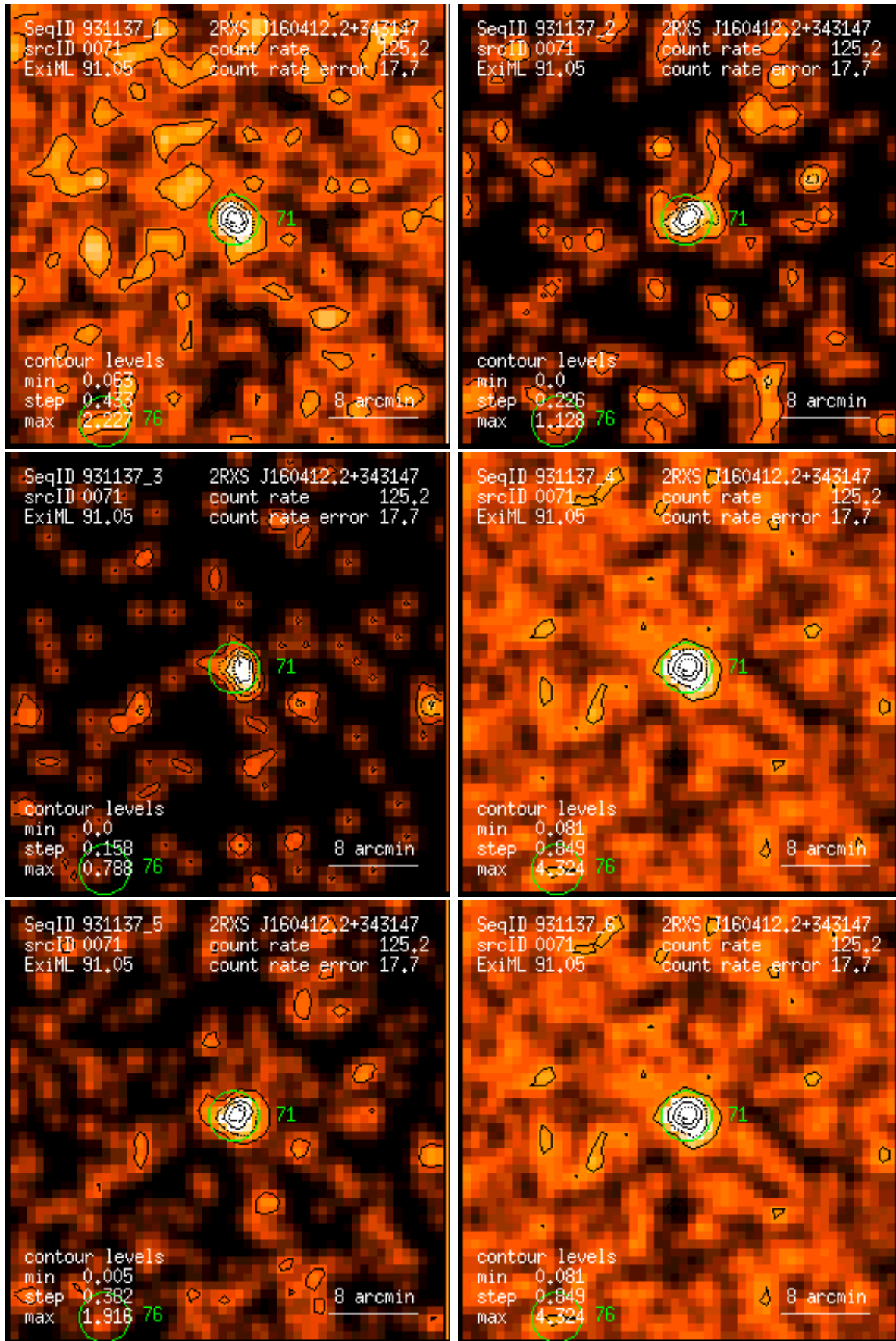
Figure 71: RASS 931137: detection 0071: band rate images, Gaussian filter: (1) PSPC channels 11 – 41, (2) 52 – 90, (3) 91 – 201, (4) 11 – 235, (5) 52 – 201, (6) 11 – 201. Broad band rates in counts/ks. Band rate contour levels in counts/ks/arcmin 2 .
