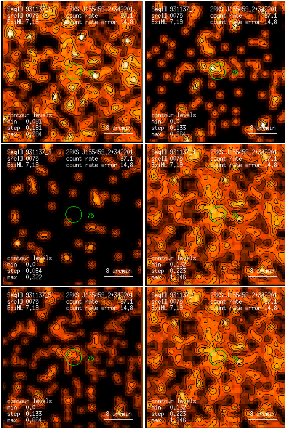
Figure 75: RASS 931137: detection 0075: band rate images, Gaussian filter: (1) PSPC channels 11 – 41, (2) 52 – 90, (3) 91 – 201, (4) 11 – 235, (5) 52 – 201, (6) 11 – 201. Broad band rates in counts/ks. Band rate contour levels in counts/ks/arcmin 2 .
