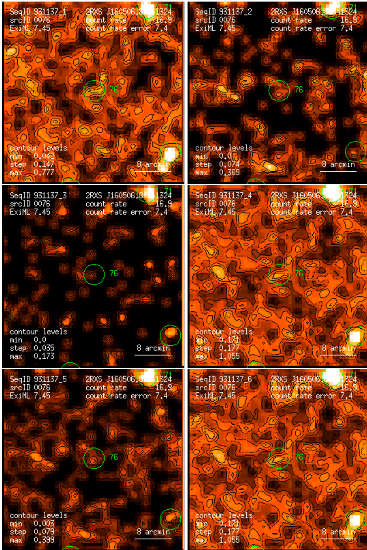
Figure 76: RASS 931137: detection 0076: band rate images, Gaussian filter: (1) PSPC channels 11 – 41, (2) 52 – 90, (3) 91 – 201, (4) 11 – 235, (5) 52 – 201, (6) 11 – 201. Broad band rates in counts/ks. Band rate contour levels in counts/ks/arcmin 2 .
