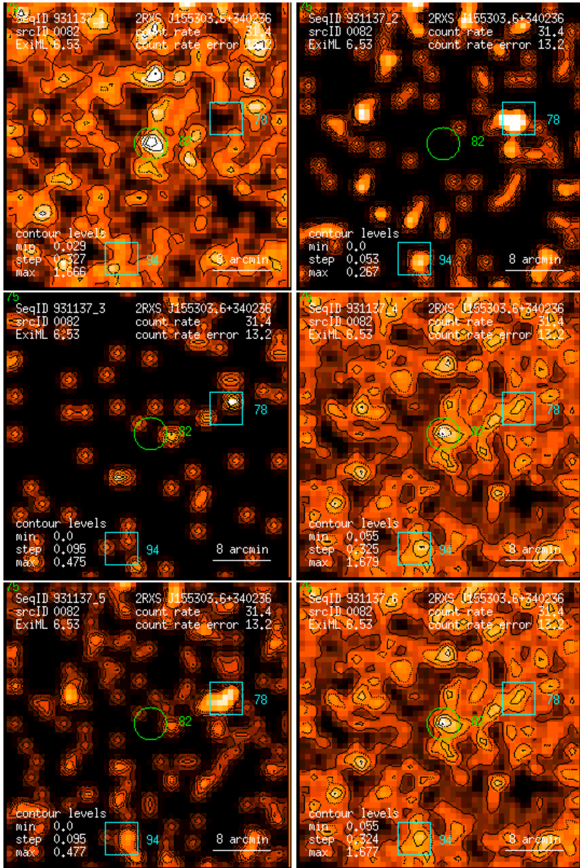
Figure 82: RASS 931137: detection 0082: band rate images, Gaussian filter: (1) PSPC channels 11 – 41, (2) 52 – 90, (3) 91 – 201, (4) 11 – 235, (5) 52 – 201, (6) 11 – 201. Broad band rates in counts/ks. Band rate contour levels in counts/ks/arcmin 2 .
