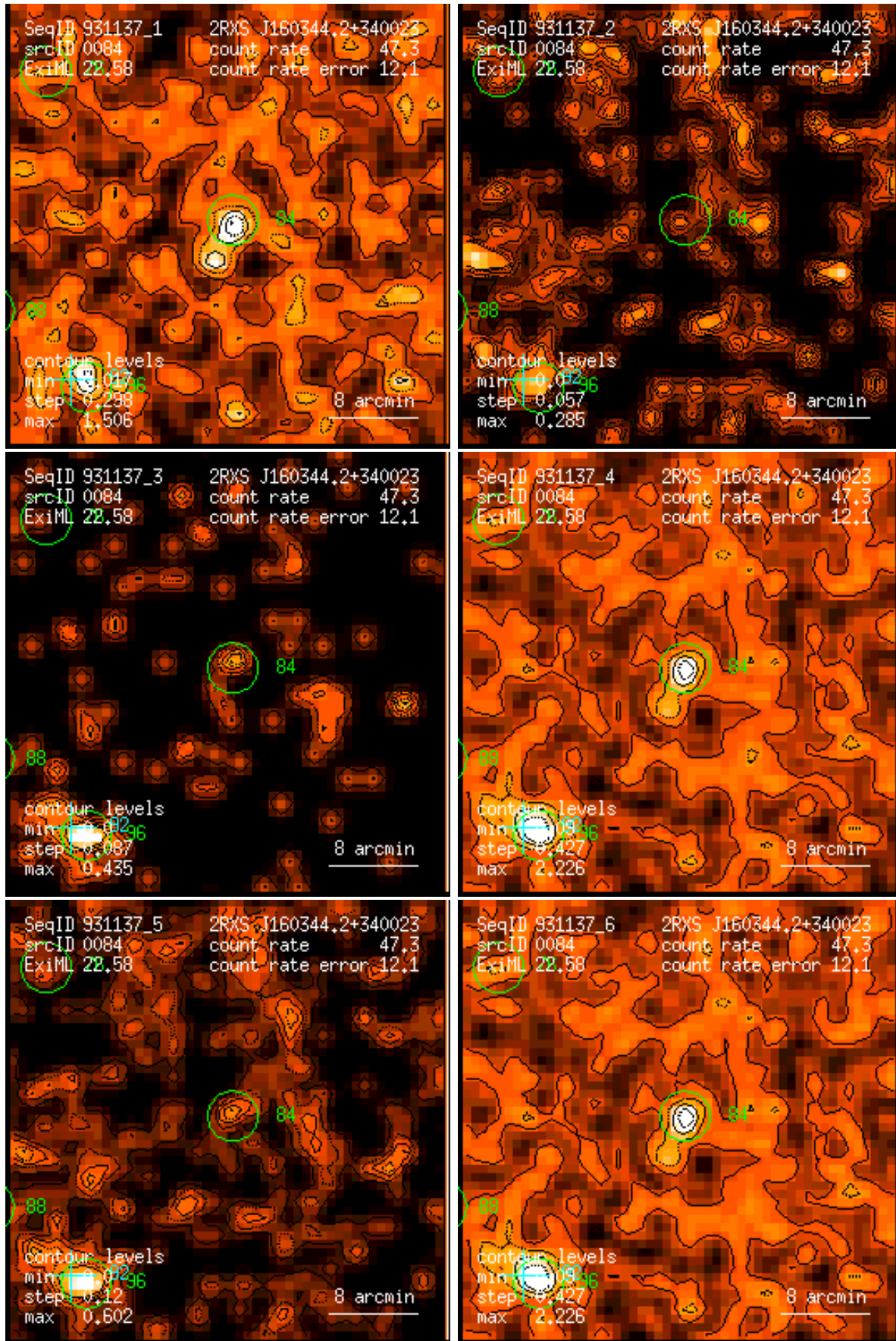
Figure 84: RASS 931137: detection 0084: band rate images, Gaussian filter: (1) PSPC channels 11 – 41, (2) 52 – 90, (3) 91 – 201, (4) 11 – 235, (5) 52 – 201, (6) 11 – 201. Broad band rates in counts/ks. Band rate contour levels in counts/ks/arcmin 2 .
