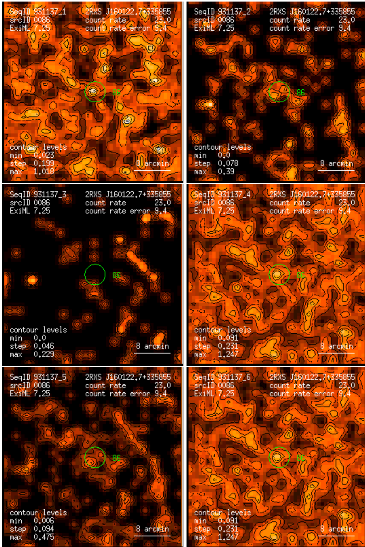
Figure 86: RASS 931137: detection 0086: band rate images, Gaussian filter: (1) PSPC channels 11 – 41, (2) 52 – 90, (3) 91 – 201, (4) 11 – 235, (5) 52 – 201, (6) 11 – 201. Broad band rates in counts/ks. Band rate contour levels in counts/ks/arcmin 2 .
