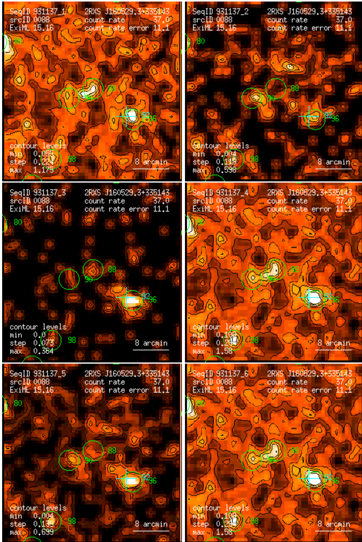
Figure 88: RASS 931137: detection 0088: band rate images, Gaussian filter: (1) PSPC channels 11 – 41, (2) 52 – 90, (3) 91 – 201, (4) 11 – 235, (5) 52 – 201, (6) 11 – 201. Broad band rates in counts/ks. Band rate contour levels in counts/ks/arcmin 2 .
