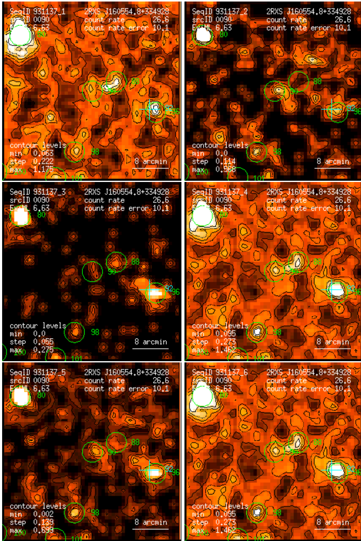
Figure 90: RASS 931137: detection 0090: band rate images, Gaussian filter: (1) PSPC channels 11 – 41, (2) 52 – 90, (3) 91 – 201, (4) 11 – 235, (5) 52 – 201, (6) 11 – 201. Broad band rates in counts/ks. Band rate contour levels in counts/ks/arcmin 2 .
