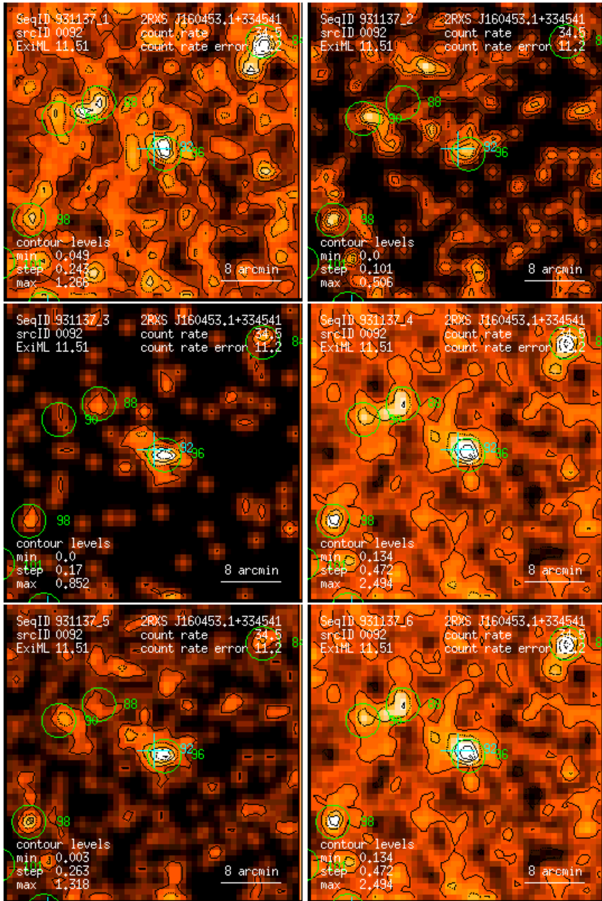
Figure 92: RASS 931137: detection 0092: band rate images, Gaussian filter: (1) PSPC channels 11 – 41, (2) 52 – 90, (3) 91 – 201, (4) 11 – 235, (5) 52 – 201, (6) 11 – 201. Broad band rates in counts/ks. Band rate contour levels in counts/ks/arcmin 2 .
