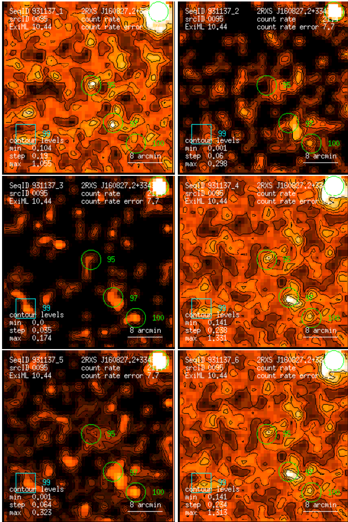
Figure 95: RASS 931137: detection 0095: band rate images, Gaussian filter: (1) PSPC channels 11 – 41, (2) 52 – 90, (3) 91 – 201, (4) 11 – 235, (5) 52 – 201, (6) 11 – 201. Broad band rates in counts/ks. Band rate contour levels in counts/ks/arcmin 2 .
