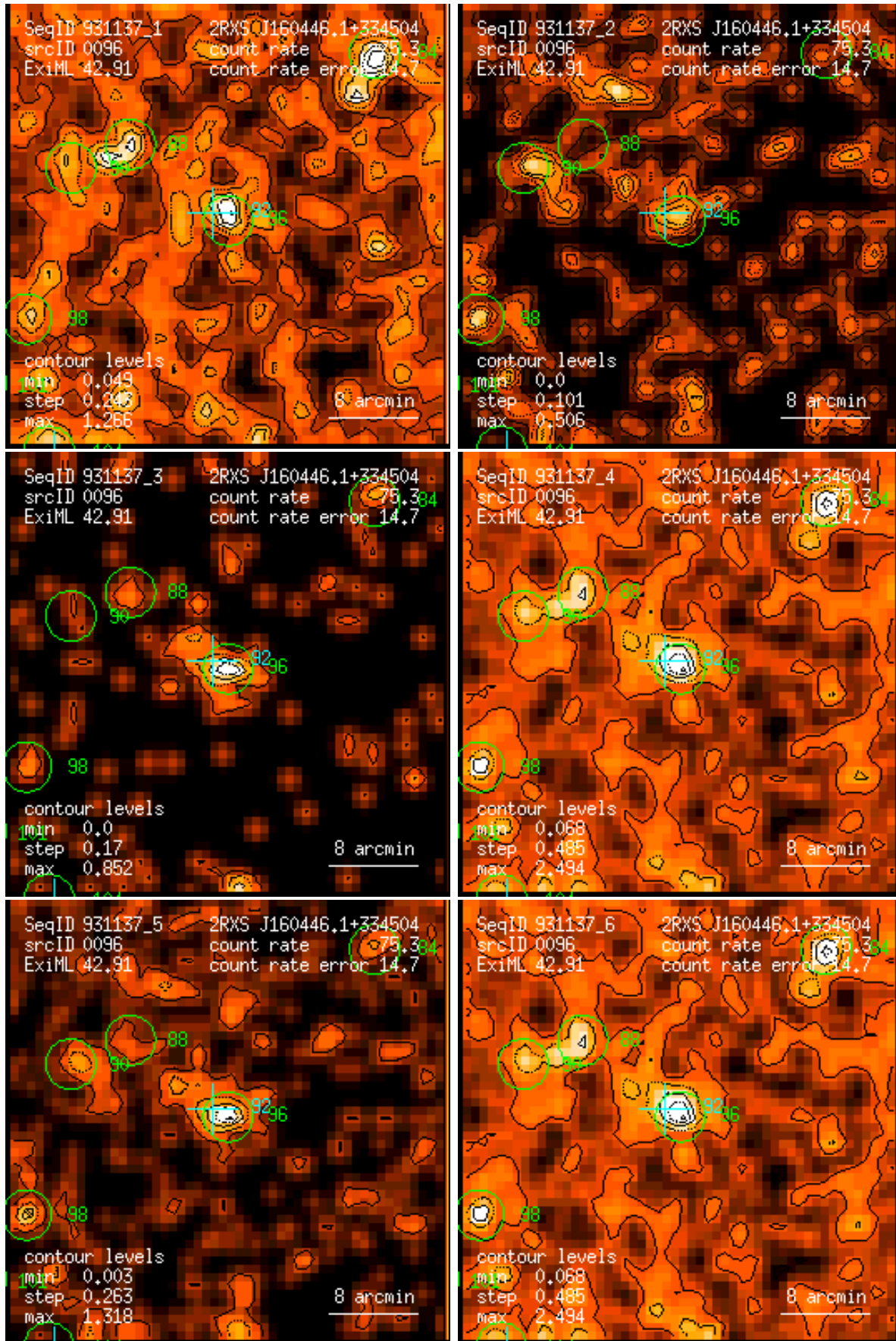
Figure 96: RASS 931137: detection 0096: band rate images, Gaussian filter: (1) PSPC channels 11 – 41, (2) 52 – 90, (3) 91 – 201, (4) 11 – 235, (5) 52 – 201, (6) 11 – 201. Broad band rates in counts/ks. Band rate contour levels in counts/ks/arcmin 2 .
