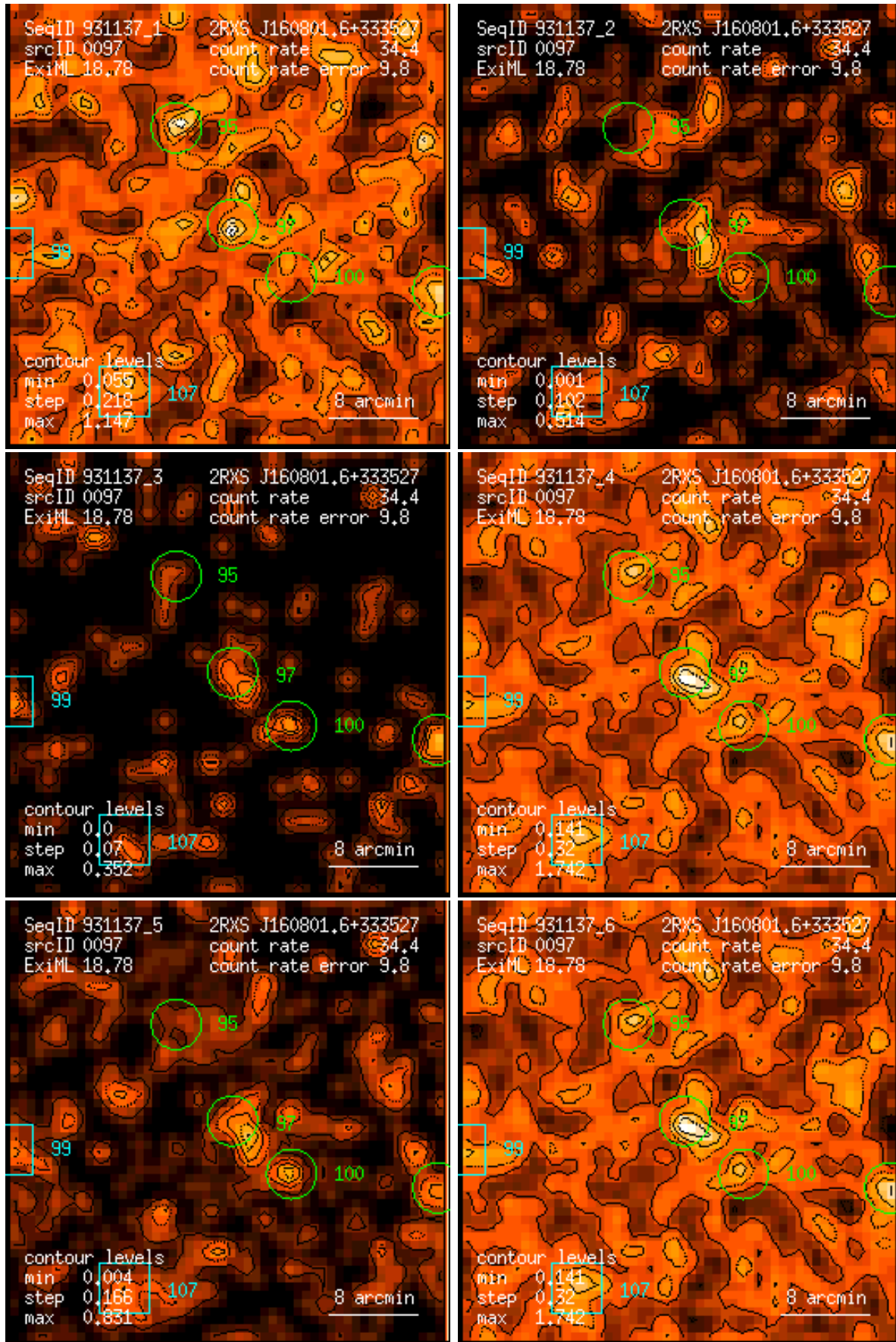
Figure 97: RASS 931137: detection 0097: band rate images, Gaussian filter: (1) PSPC channels 11 – 41, (2) 52 – 90, (3) 91 – 201, (4) 11 – 235, (5) 52 – 201, (6) 11 – 201. Broad band rates in counts/ks. Band rate contour levels in counts/ks/arcmin 2 .
