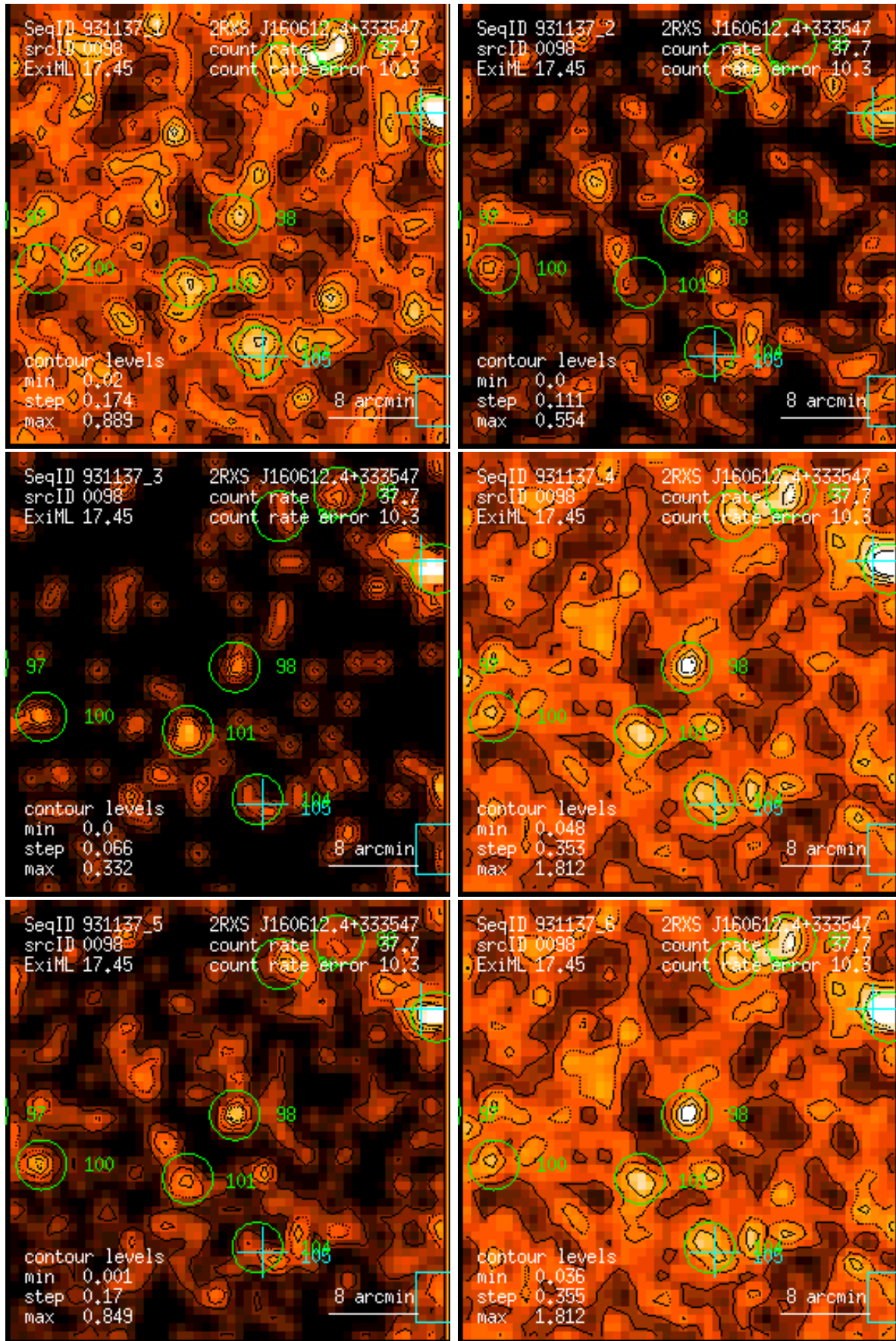
Figure 98: RASS 931137: detection 0098: band rate images, Gaussian filter: (1) PSPC channels 11 – 41, (2) 52 – 90, (3) 91 – 201, (4) 11 – 235, (5) 52 – 201, (6) 11 – 201. Broad band rates in counts/ks. Band rate contour levels in counts/ks/arcmin 2 .
