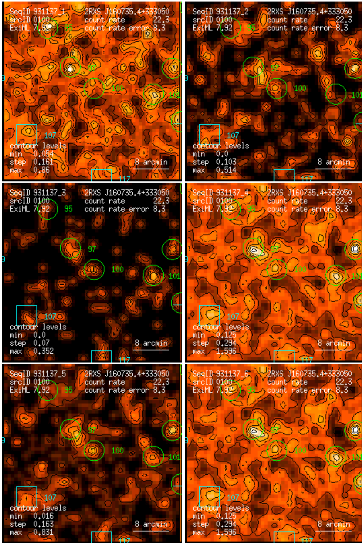
Figure 100: RASS 931137: detection 0100: band rate images, Gaussian filter: (1) PSPC channels 11 – 41, (2) 52 – 90, (3) 91 – 201, (4) 11 – 235, (5) 52 – 201, (6) 11 – 201. Broad band rates in counts/ks. Band rate contour levels in counts/ks/arcmin 2 .
