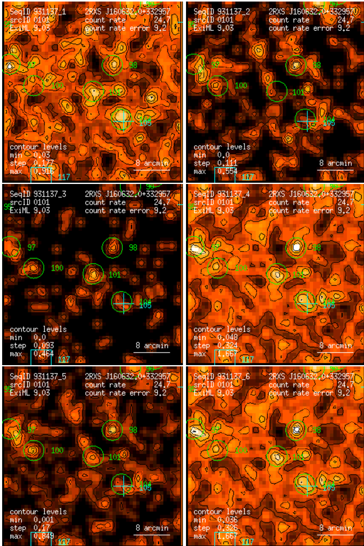
Figure 101: RASS 931137: detection 0101: band rate images, Gaussian filter: (1) PSPC channels 11 – 41, (2) 52 – 90, (3) 91 – 201, (4) 11 – 235, (5) 52 – 201, (6) 11 – 201. Broad band rates in counts/ks. Band rate contour levels in counts/ks/arcmin 2 .
