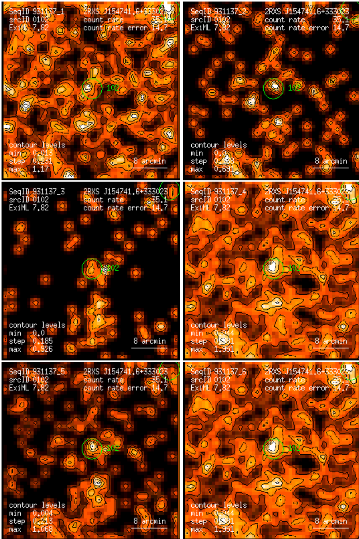
Figure 102: RASS 931137: detection 0102: band rate images, Gaussian filter: (1) PSPC channels 11 – 41, (2) 52 – 90, (3) 91 – 201, (4) 11 – 235, (5) 52 – 201, (6) 11 – 201. Broad band rates in counts/ks. Band rate contour levels in counts/ks/arcmin 2 .
