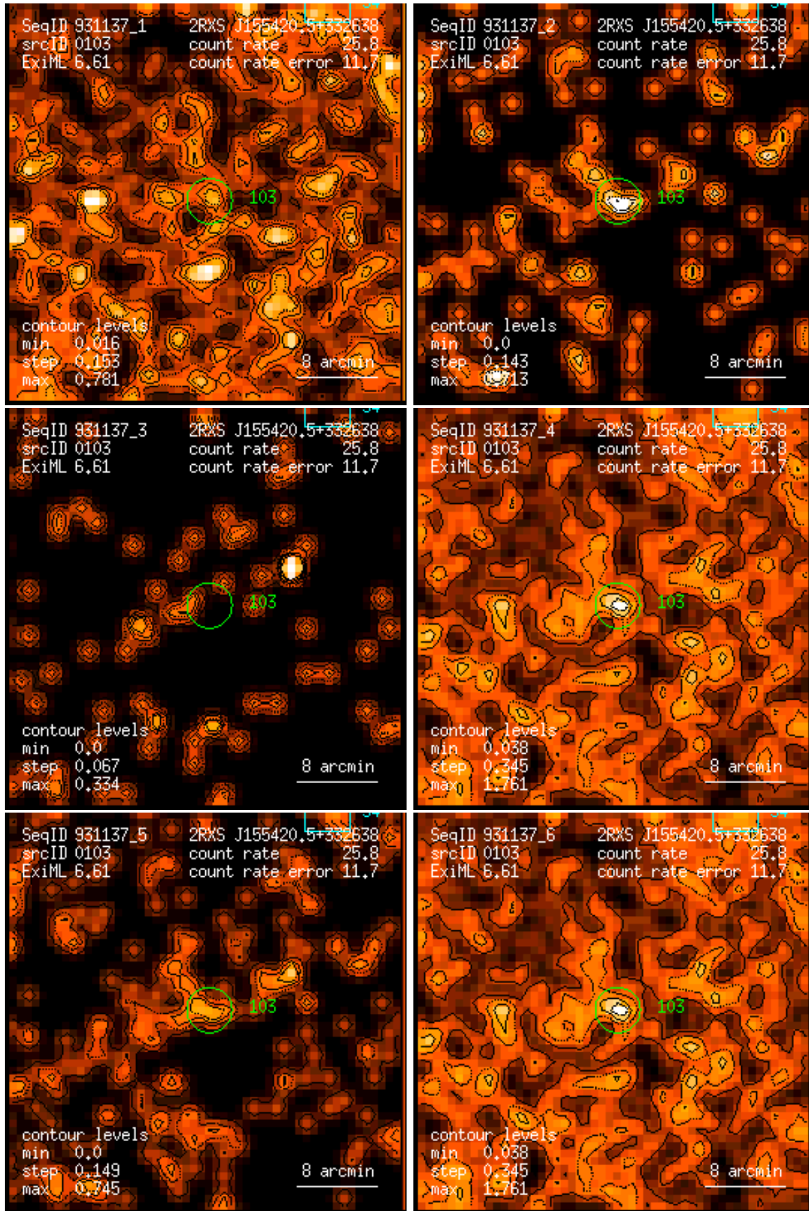
Figure 103: RASS 931137: detection 0103: band rate images, Gaussian filter: (1) PSPC channels 11 – 41, (2) 52 – 90, (3) 91 – 201, (4) 11 – 235, (5) 52 – 201, (6) 11 – 201. Broad band rates in counts/ks. Band rate contour levels in counts/ks/arcmin 2 .
