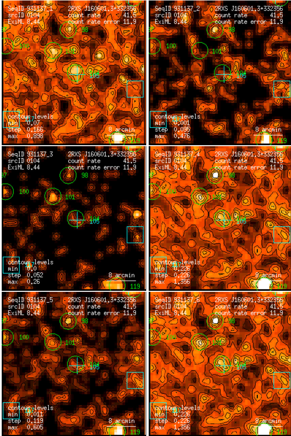
Figure 104: RASS 931137: detection 0104: band rate images, Gaussian filter: (1) PSPC channels 11 – 41, (2) 52 – 90, (3) 91 – 201, (4) 11 – 235, (5) 52 – 201, (6) 11 – 201. Broad band rates in counts/ks. Band rate contour levels in counts/ks/arcmin 2 .
