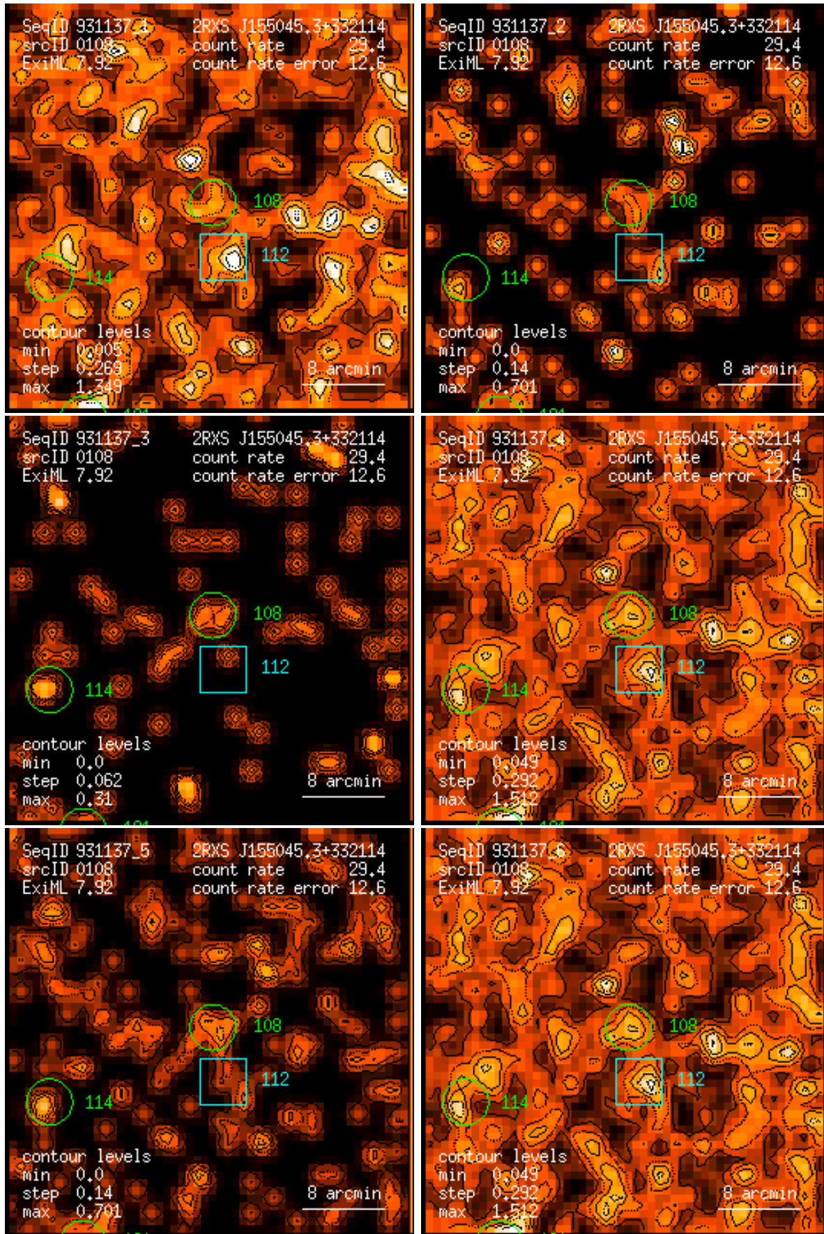
Figure 108: RASS 931137: detection 0108: band rate images, Gaussian filter: (1) PSPC channels 11 – 41, (2) 52 – 90, (3) 91 – 201, (4) 11 – 235, (5) 52 – 201, (6) 11 – 201. Broad band rates in counts/ks. Band rate contour levels in counts/ks/arcmin 2 .
