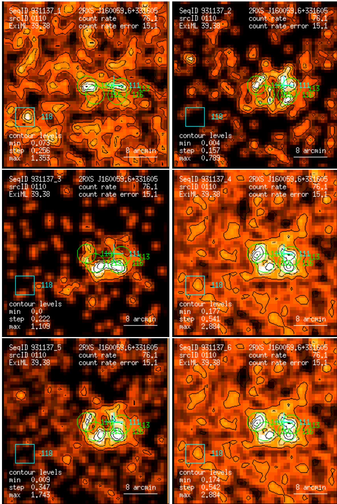
Figure 110: RASS 931137: detection 0110: band rate images, Gaussian filter: (1) PSPC channels 11 – 41, (2) 52 – 90, (3) 91 – 201, (4) 11 – 235, (5) 52 – 201, (6) 11 – 201. Broad band rates in counts/ks. Band rate contour levels in counts/ks/arcmin 2 .
