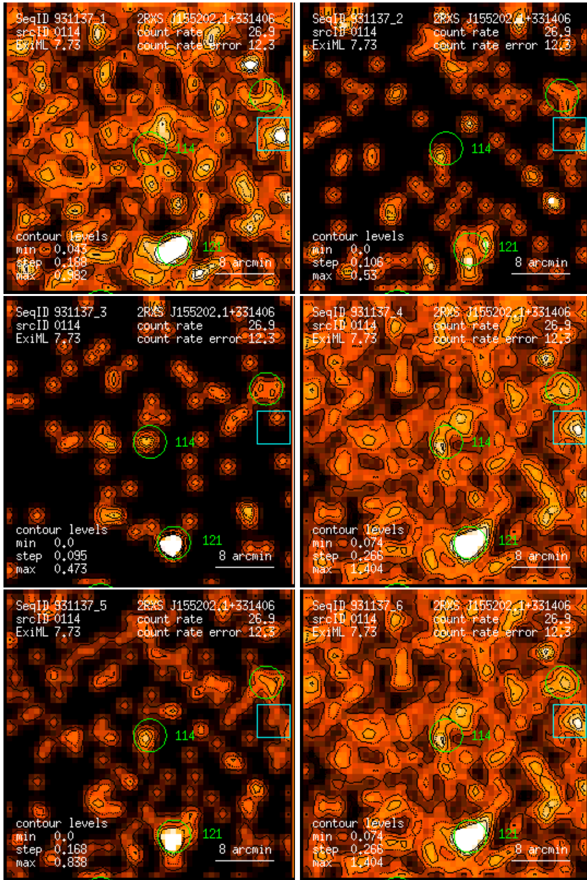
Figure 114: RASS 931137: detection 0114: band rate images, Gaussian filter: (1) PSPC channels 11 – 41, (2) 52 – 90, (3) 91 – 201, (4) 11 – 235, (5) 52 – 201, (6) 11 – 201. Broad band rates in counts/ks. Band rate contour levels in counts/ks/arcmin 2 .
