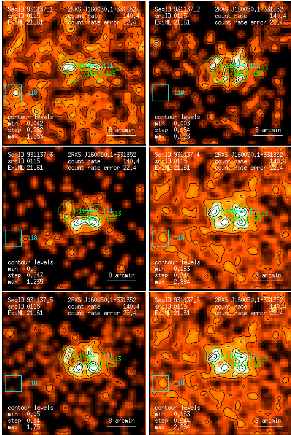
Figure 115: RASS 931137: detection 0115: band rate images, Gaussian filter: (1) PSPC channels 11 – 41, (2) 52 – 90, (3) 91 – 201, (4) 11 – 235, (5) 52 – 201, (6) 11 – 201. Broad band rates in counts/ks. Band rate contour levels in counts/ks/arcmin 2 .
