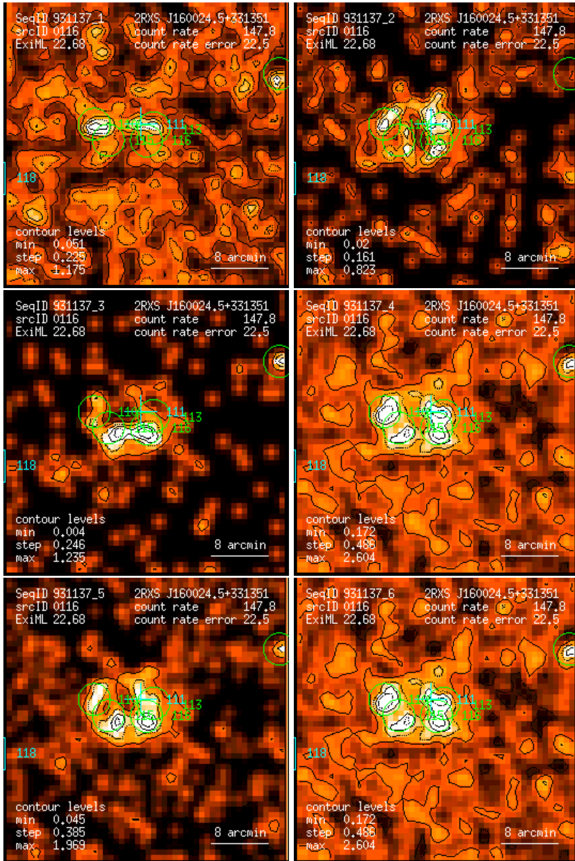
Figure 116: RASS 931137: detection 0116: band rate images, Gaussian filter: (1) PSPC channels 11 – 41, (2) 52 – 90, (3) 91 – 201, (4) 11 – 235, (5) 52 – 201, (6) 11 – 201. Broad band rates in counts/ks. Band rate contour levels in counts/ks/arcmin 2 .
