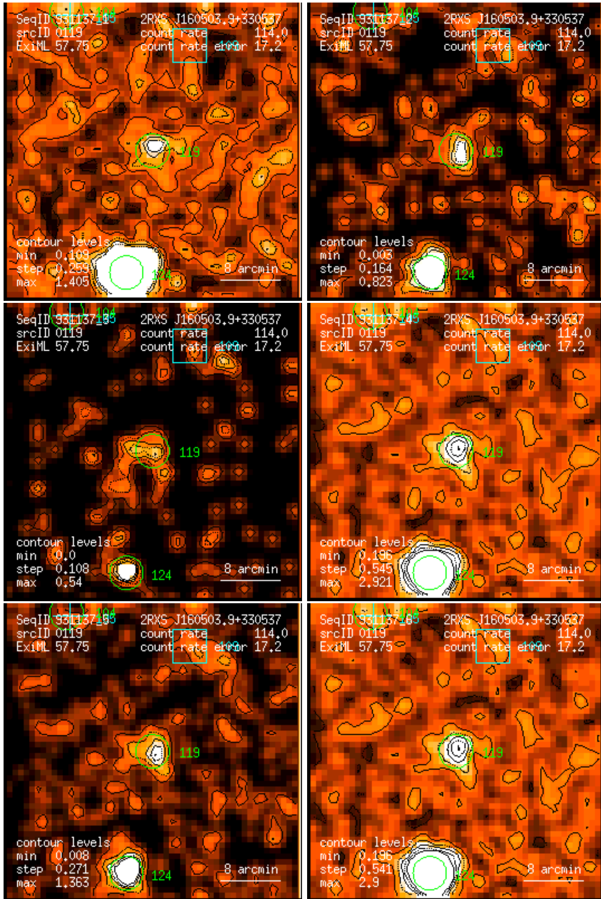
Figure 119: RASS 931137: detection 0119: band rate images, Gaussian filter: (1) PSPC channels 11 – 41, (2) 52 – 90, (3) 91 – 201, (4) 11 – 235, (5) 52 – 201, (6) 11 – 201. Broad band rates in counts/ks. Band rate contour levels in counts/ks/arcmin 2 .
