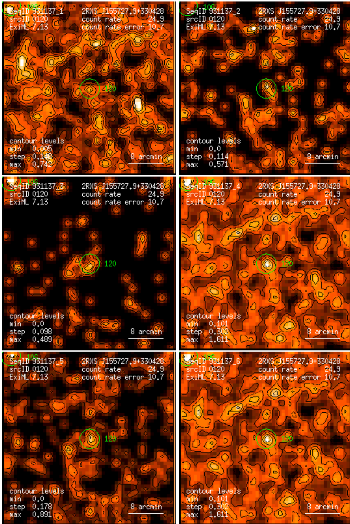
Figure 120: RASS 931137: detection 0120: band rate images, Gaussian filter: (1) PSPC channels 11 – 41, (2) 52 – 90, (3) 91 – 201, (4) 11 – 235, (5) 52 – 201, (6) 11 – 201. Broad band rates in counts/ks. Band rate contour levels in counts/ks/arcmin 2 .
