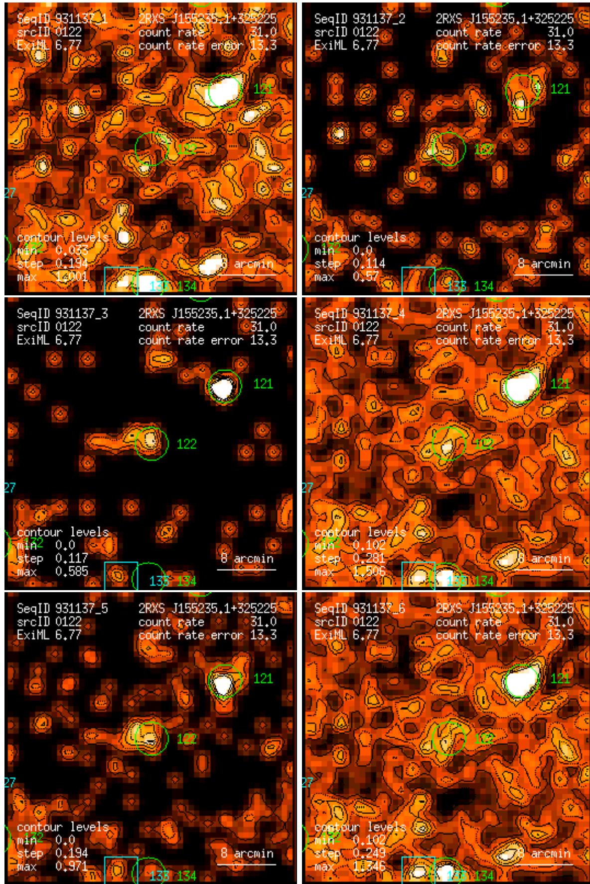
Figure 122: RASS 931137: detection 0122: band rate images, Gaussian filter: (1) PSPC channels 11 – 41, (2) 52 – 90, (3) 91 – 201, (4) 11 – 235, (5) 52 – 201, (6) 11 – 201. Broad band rates in counts/ks. Band rate contour levels in counts/ks/arcmin 2 .
