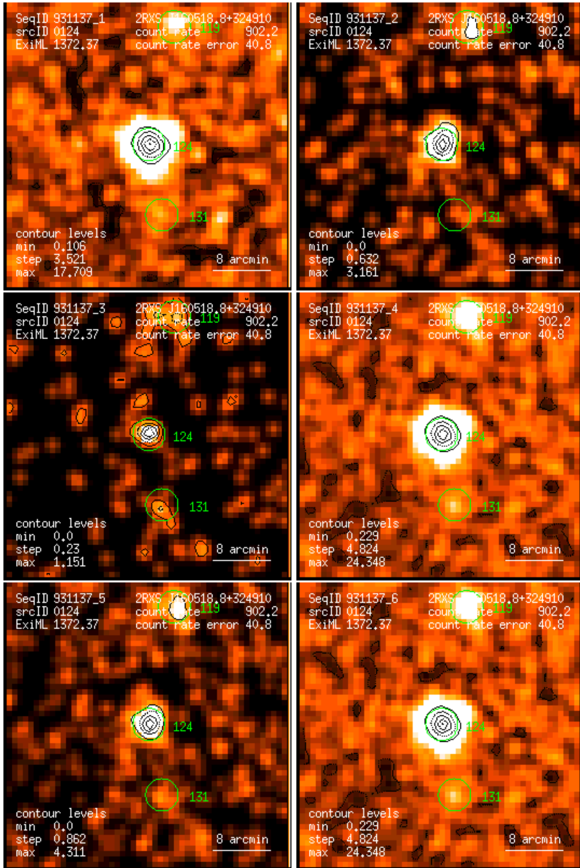
Figure 124: RASS 931137: detection 0124: band rate images, Gaussian filter: (1) PSPC channels 11 – 41, (2) 52 – 90, (3) 91 – 201, (4) 11 – 235, (5) 52 – 201, (6) 11 – 201. Broad band rates in counts/ks. Band rate contour levels in counts/ks/arcmin 2 .
