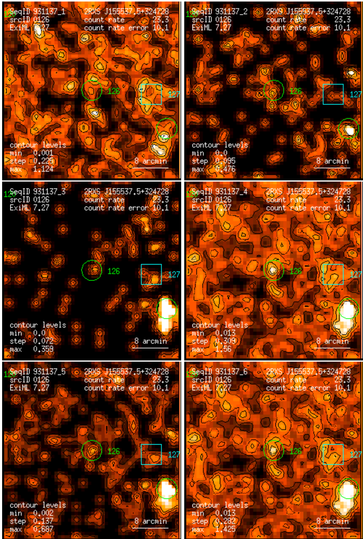
Figure 126: RASS 931137: detection 0126: band rate images, Gaussian filter: (1) PSPC channels 11 – 41, (2) 52 – 90, (3) 91 – 201, (4) 11 – 235, (5) 52 – 201, (6) 11 – 201. Broad band rates in counts/ks. Band rate contour levels in counts/ks/arcmin 2 .
