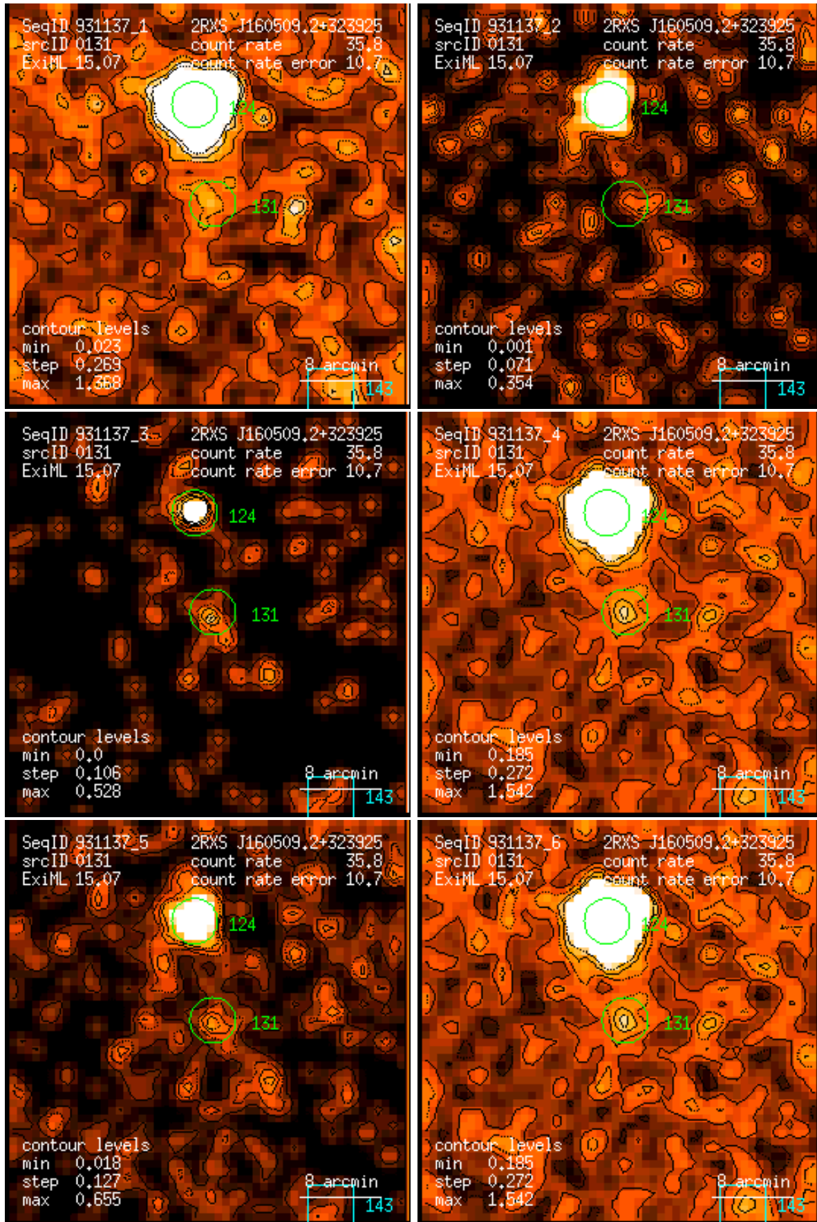
Figure 131: RASS 931137: detection 0131: band rate images, Gaussian filter: (1) PSPC channels 11 – 41, (2) 52 – 90, (3) 91 – 201, (4) 11 – 235, (5) 52 – 201, (6) 11 – 201. Broad band rates in counts/ks. Band rate contour levels in counts/ks/arcmin 2 .
