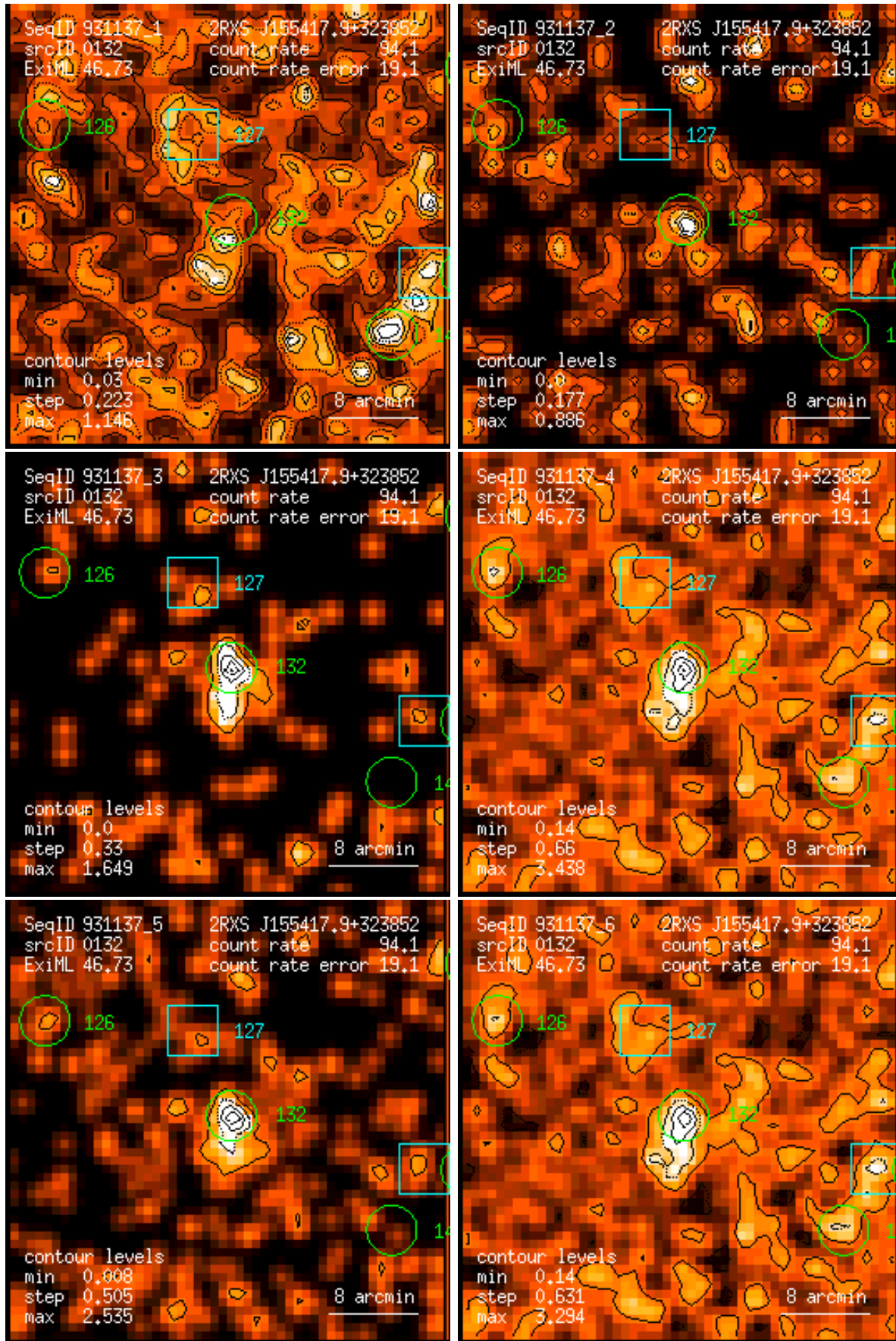
Figure 132: RASS 931137: detection 0132: band rate images, Gaussian filter: (1) PSPC channels 11 – 41, (2) 52 – 90, (3) 91 – 201, (4) 11 – 235, (5) 52 – 201, (6) 11 – 201. Broad band rates in counts/ks. Band rate contour levels in counts/ks/arcmin 2 .
