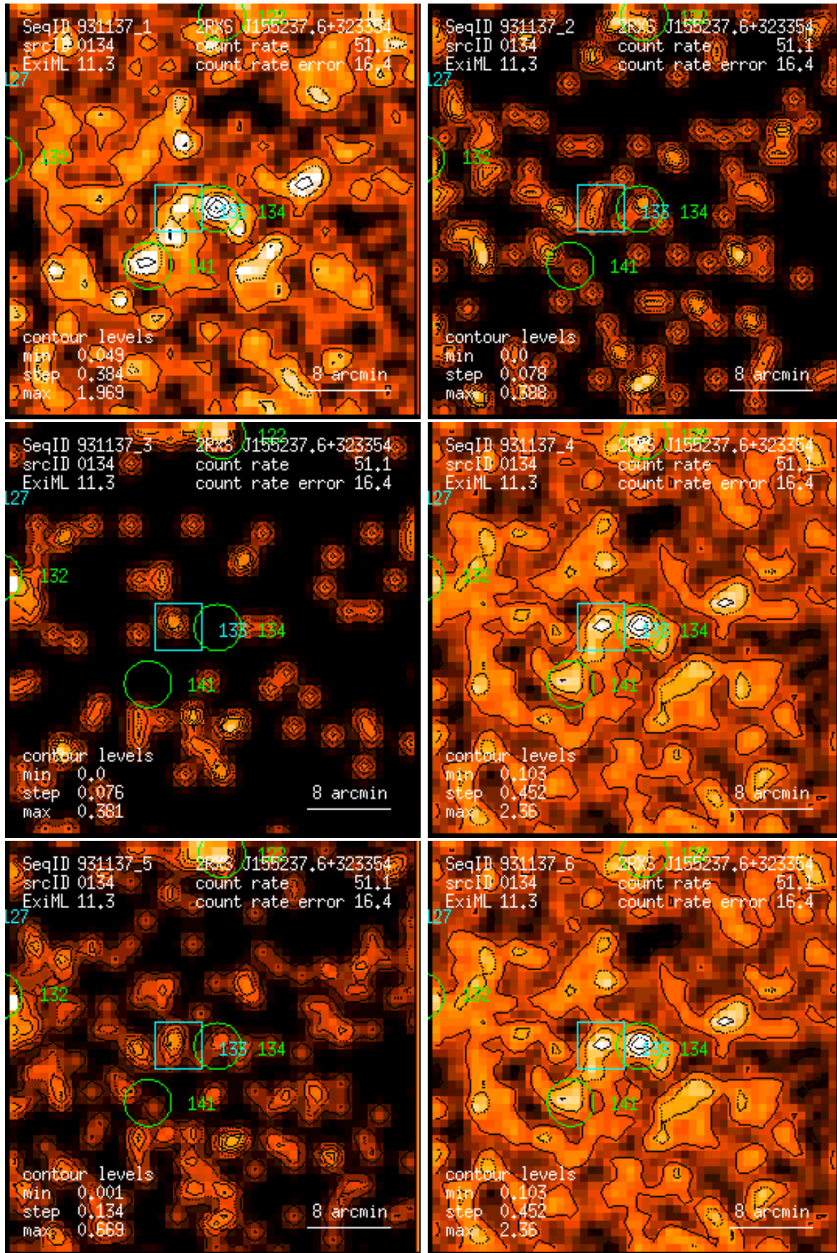
Figure 134: RASS 931137: detection 0134: band rate images, Gaussian filter: (1) PSPC channels 11 – 41, (2) 52 – 90, (3) 91 – 201, (4) 11 – 235, (5) 52 – 201, (6) 11 – 201. Broad band rates in counts/ks. Band rate contour levels in counts/ks/arcmin 2 .
