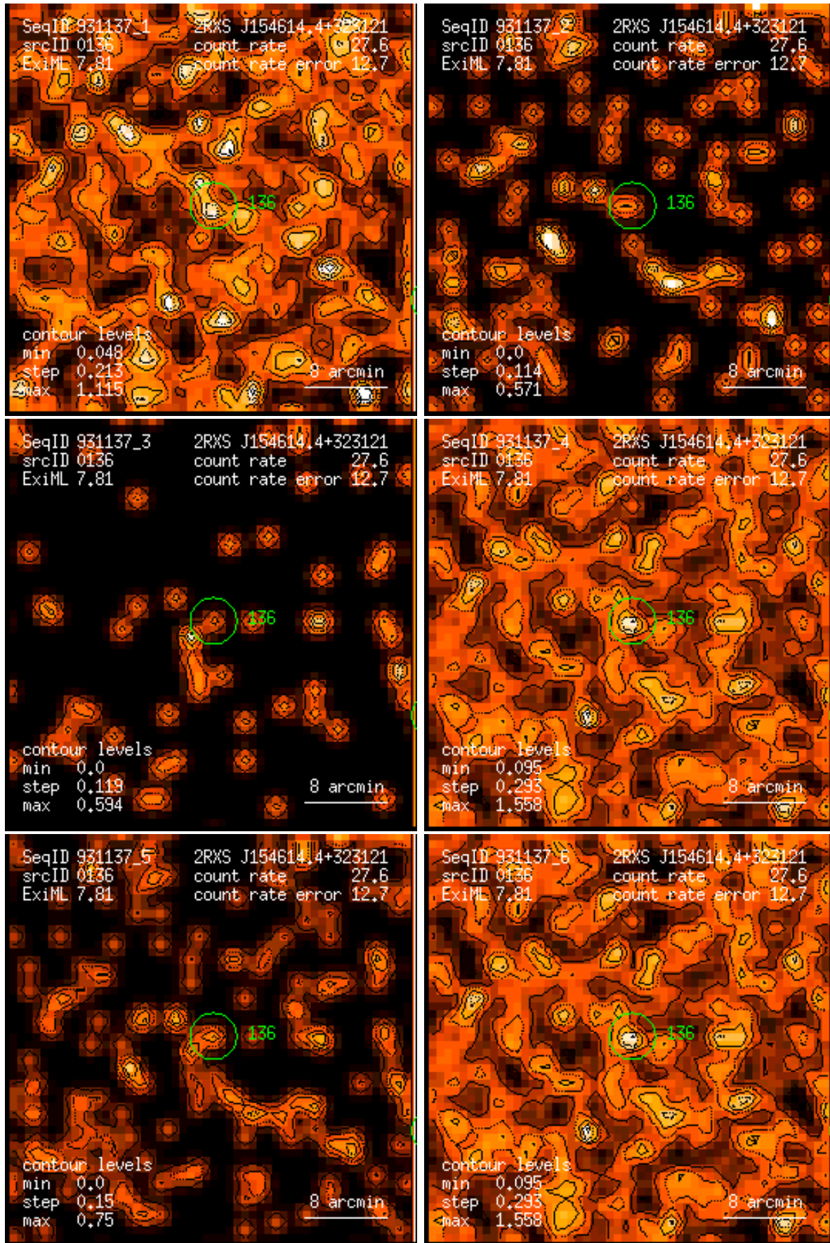
Figure 136: RASS 931137: detection 0136: band rate images, Gaussian filter: (1) PSPC channels 11 – 41, (2) 52 – 90, (3) 91 – 201, (4) 11 – 235, (5) 52 – 201, (6) 11 – 201. Broad band rates in counts/ks. Band rate contour levels in counts/ks/arcmin 2 .
