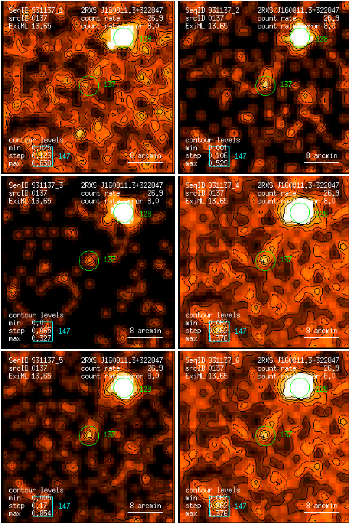
Figure 137: RASS 931137: detection 0137: band rate images, Gaussian filter: (1) PSPC channels 11 – 41, (2) 52 – 90, (3) 91 – 201, (4) 11 – 235, (5) 52 – 201, (6) 11 – 201. Broad band rates in counts/ks. Band rate contour levels in counts/ks/arcmin 2 .
