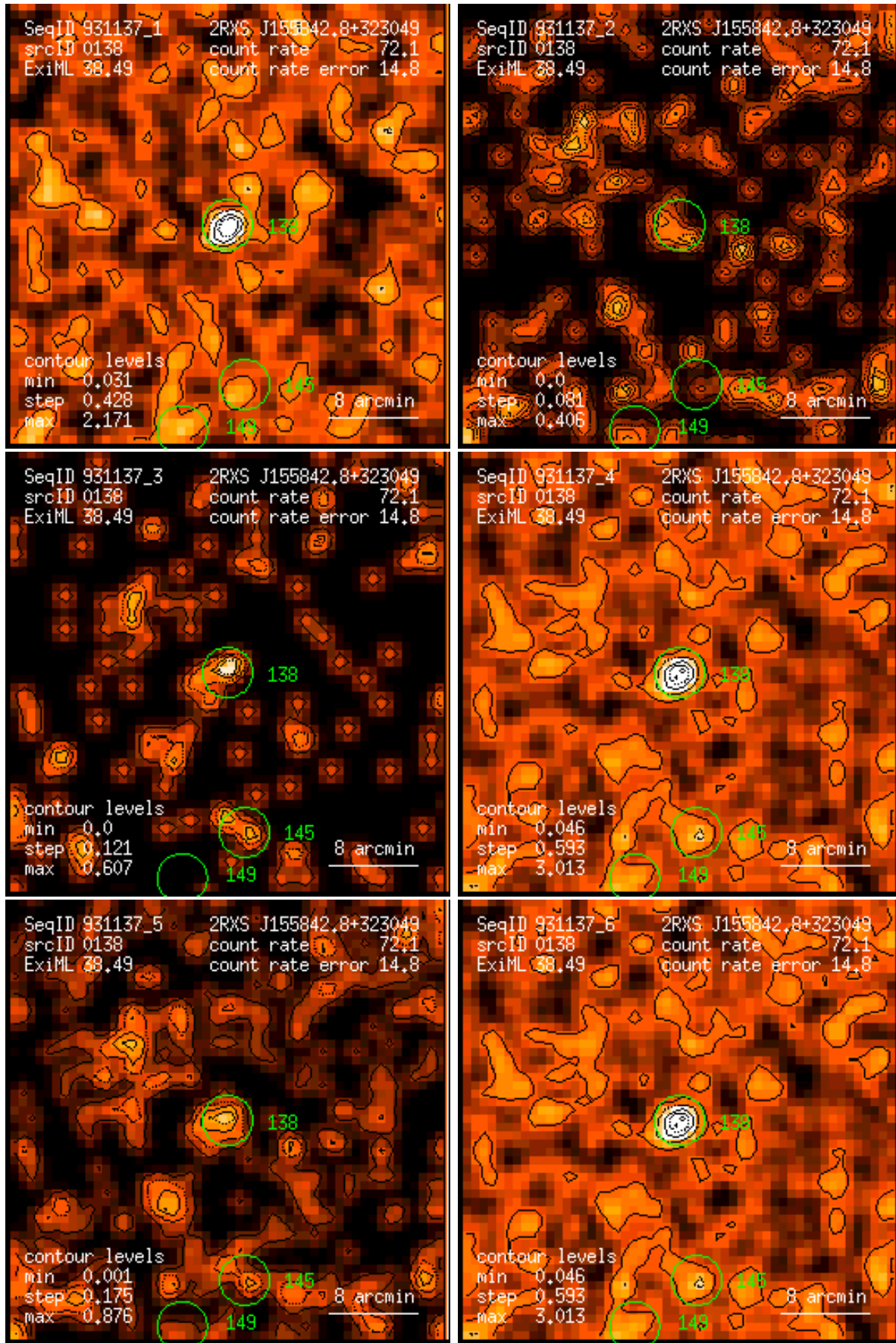
Figure 138: RASS 931137: detection 0138: band rate images, Gaussian filter: (1) PSPC channels 11 – 41, (2) 52 – 90, (3) 91 – 201, (4) 11 – 235, (5) 52 – 201, (6) 11 – 201. Broad band rates in counts/ks. Band rate contour levels in counts/ks/arcmin 2 .
