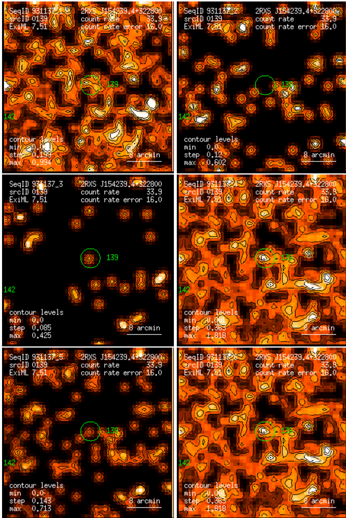
Figure 139: RASS 931137: detection 0139: band rate images, Gaussian filter: (1) PSPC channels 11 – 41, (2) 52 – 90, (3) 91 – 201, (4) 11 – 235, (5) 52 – 201, (6) 11 – 201. Broad band rates in counts/ks. Band rate contour levels in counts/ks/arcmin 2 .
