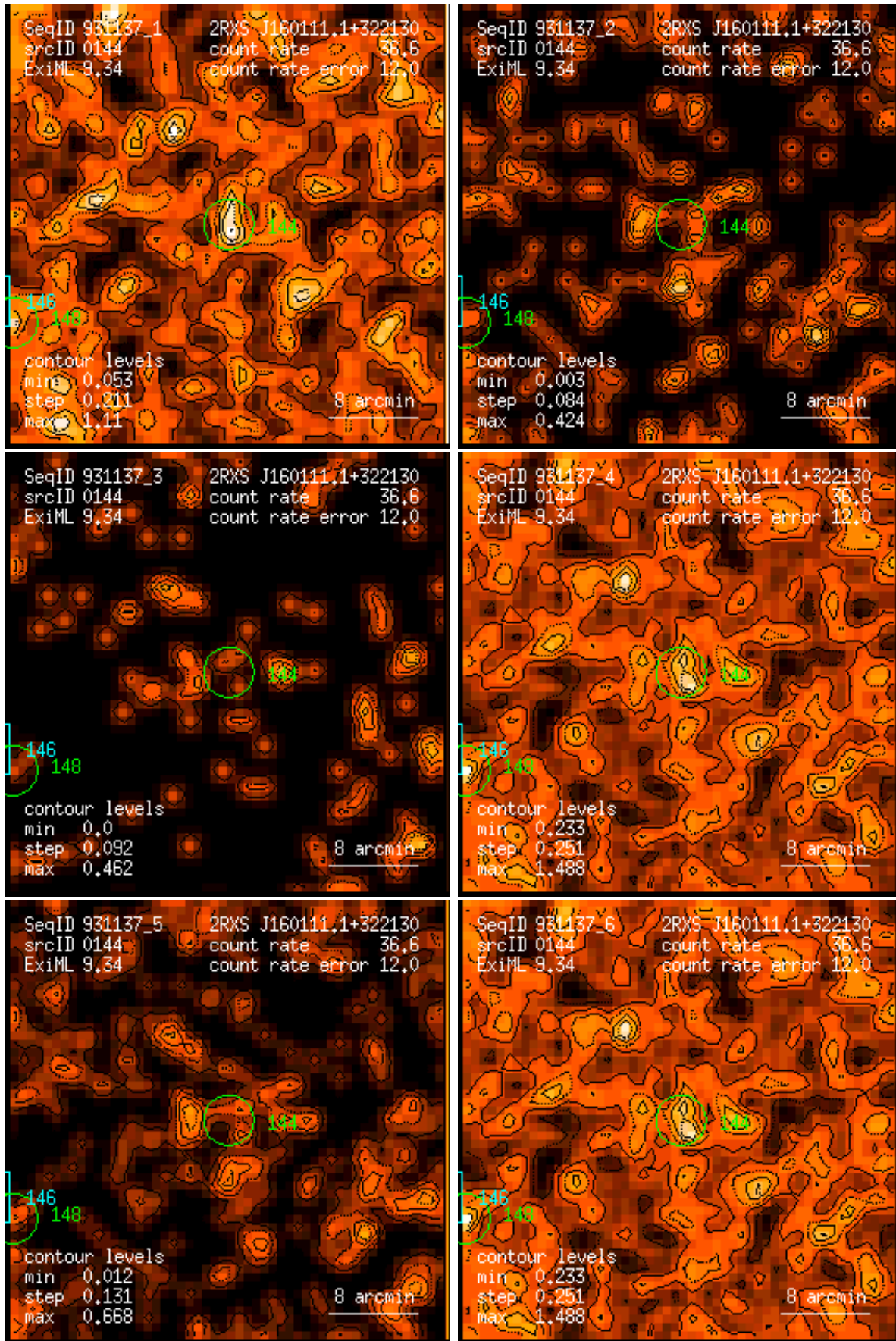
Figure 144: RASS 931137: detection 0144: band rate images, Gaussian filter: (1) PSPC channels 11 – 41, (2) 52 – 90, (3) 91 – 201, (4) 11 – 235, (5) 52 – 201, (6) 11 – 201. Broad band rates in counts/ks. Band rate contour levels in counts/ks/arcmin 2 .
