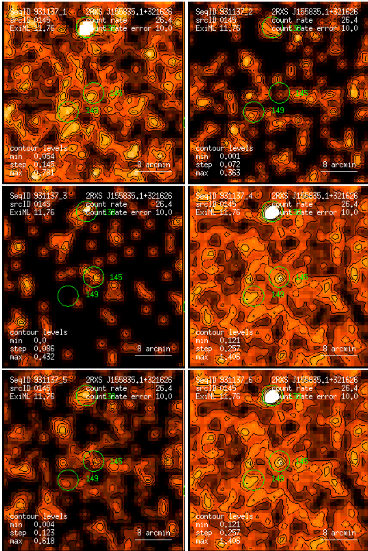
Figure 145: RASS 931137: detection 0145: band rate images, Gaussian filter: (1) PSPC channels 11 – 41, (2) 52 – 90, (3) 91 – 201, (4) 11 – 235, (5) 52 – 201, (6) 11 – 201. Broad band rates in counts/ks. Band rate contour levels in counts/ks/arcmin 2 .
