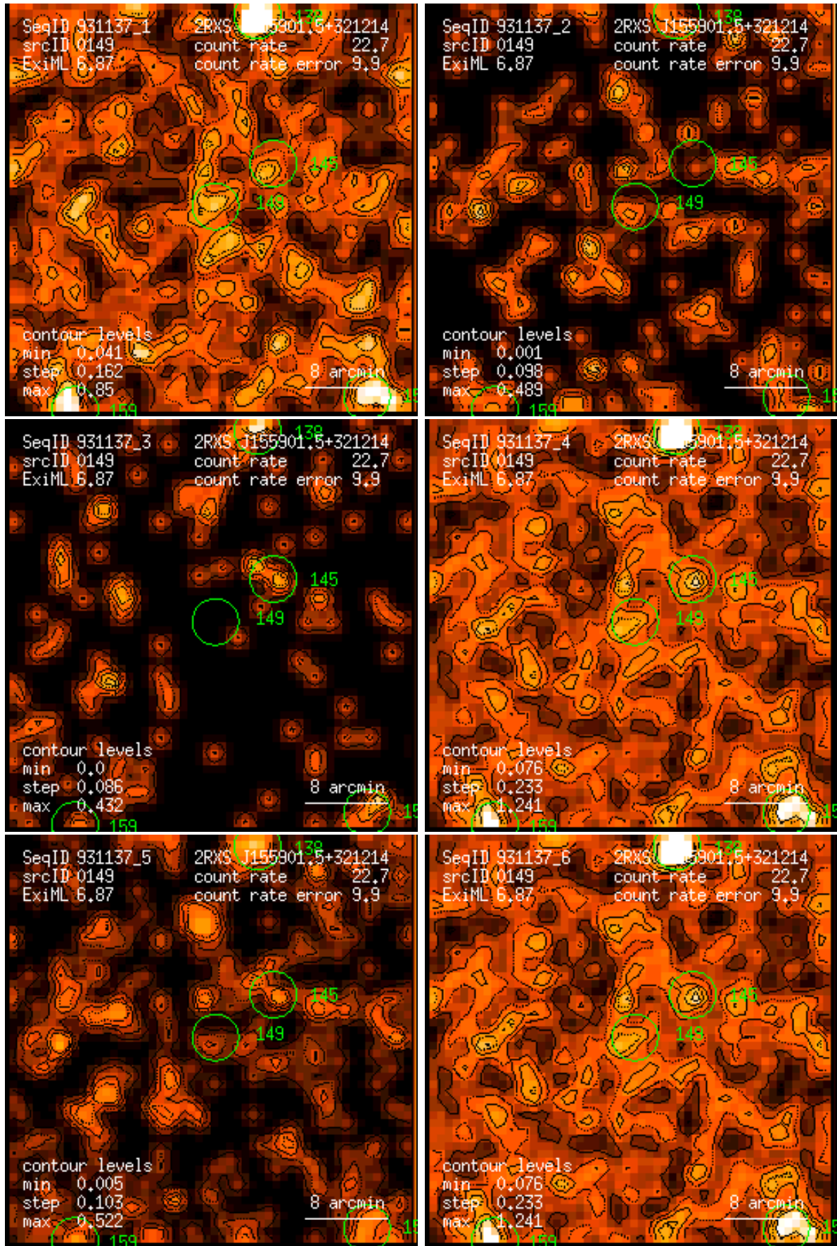
Figure 149: RASS 931137: detection 0149: band rate images, Gaussian filter: (1) PSPC channels 11 – 41, (2) 52 – 90, (3) 91 – 201, (4) 11 – 235, (5) 52 – 201, (6) 11 – 201. Broad band rates in counts/ks. Band rate contour levels in counts/ks/arcmin 2 .
