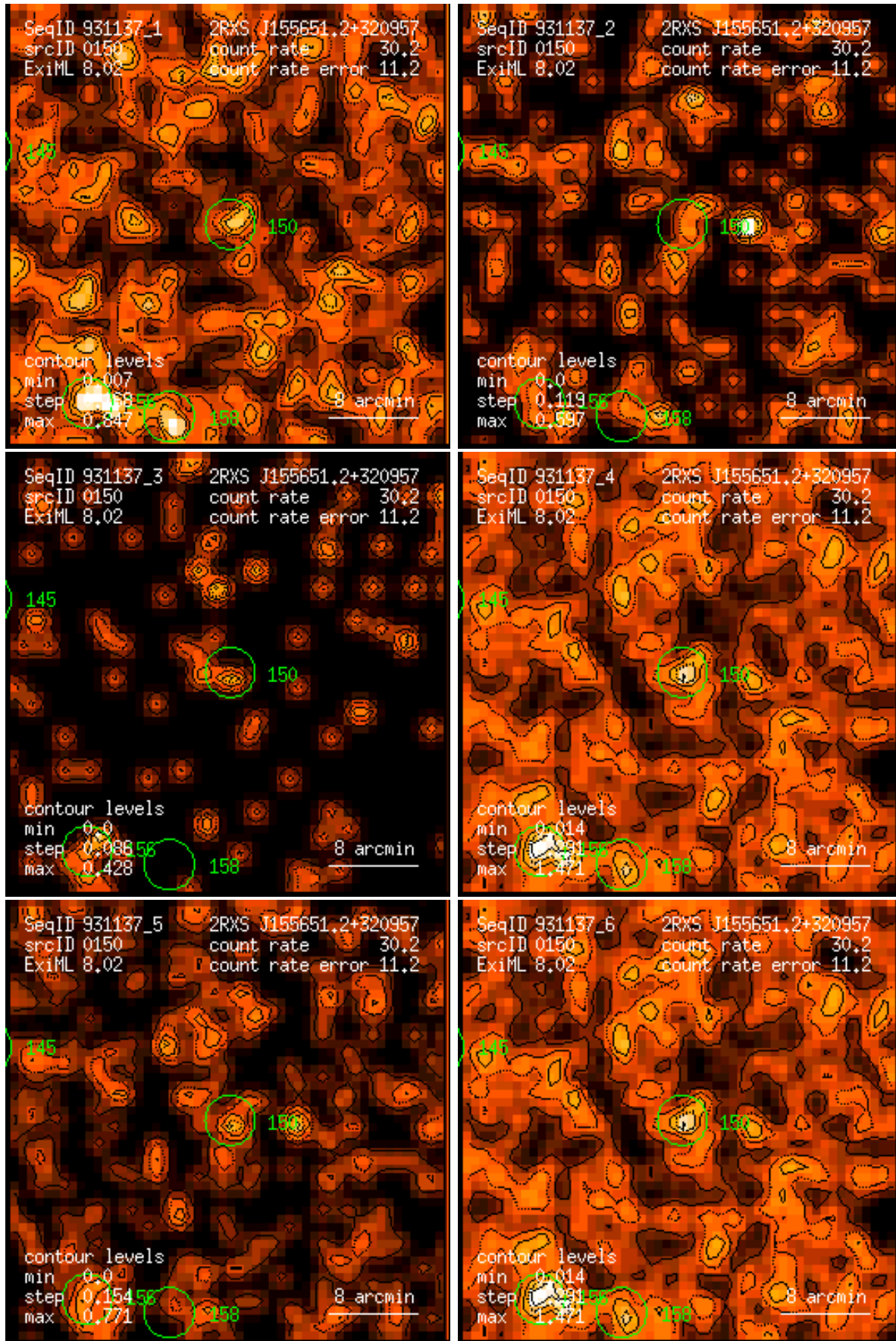
Figure 150: RASS 931137: detection 0150: band rate images, Gaussian filter: (1) PSPC channels 11 – 41, (2) 52 – 90, (3) 91 – 201, (4) 11 – 235, (5) 52 – 201, (6) 11 – 201. Broad band rates in counts/ks. Band rate contour levels in counts/ks/arcmin 2 .
